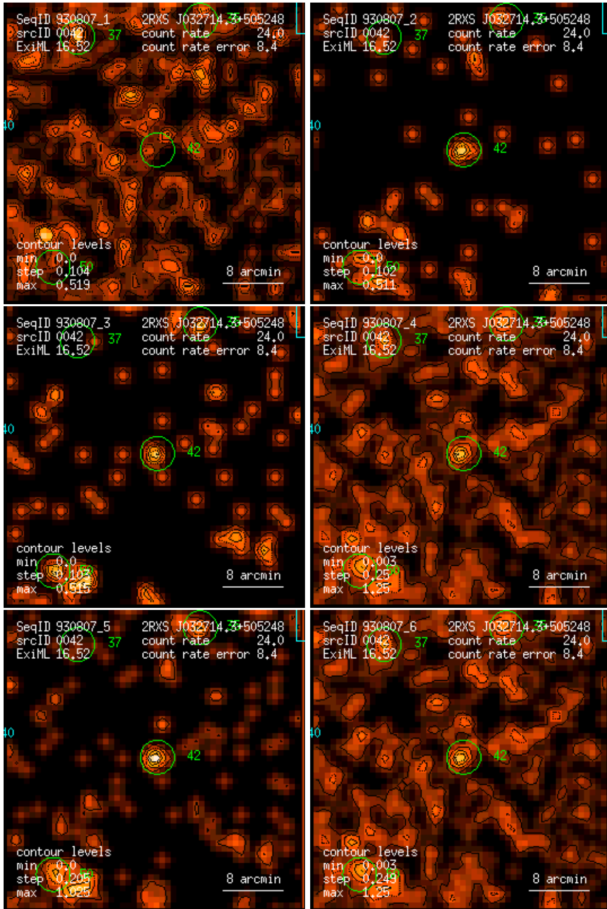
Figure 42: RASS 930807: detection 0042: band rate images, Gaussian filter: (1) PSPC channels 11 – 41, (2) 52 – 90, (3) 91 – 201, (4) 11 – 235, (5) 52 – 201, (6) 11 – 201. Broad band rates in counts/ks. Band rate contour levels in counts/ks/arcmin 2 .
