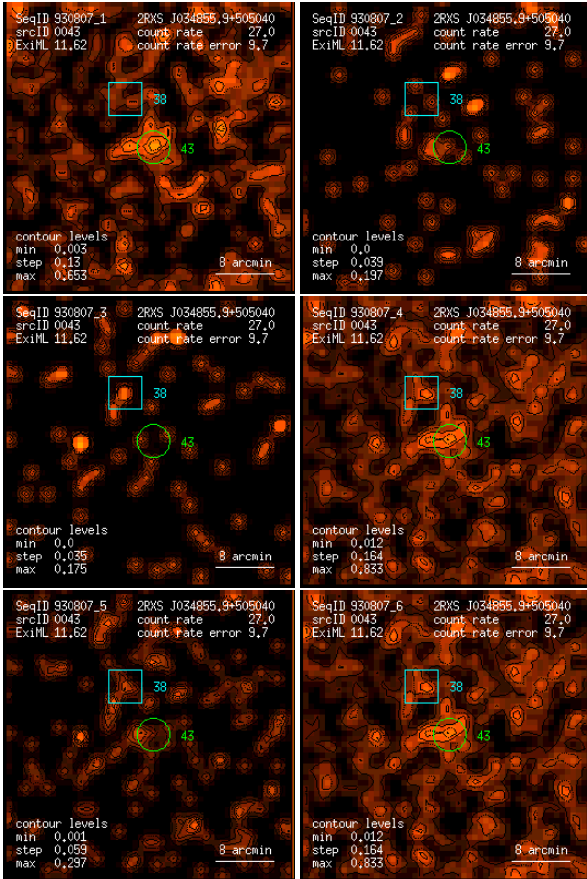
Figure 43: RASS 930807: detection 0043: band rate images, Gaussian filter: (1) PSPC channels 11 – 41, (2) 52 – 90, (3) 91 – 201, (4) 11 – 235, (5) 52 – 201, (6) 11 – 201. Broad band rates in counts/ks. Band rate contour levels in counts/ks/arcmin 2 .
