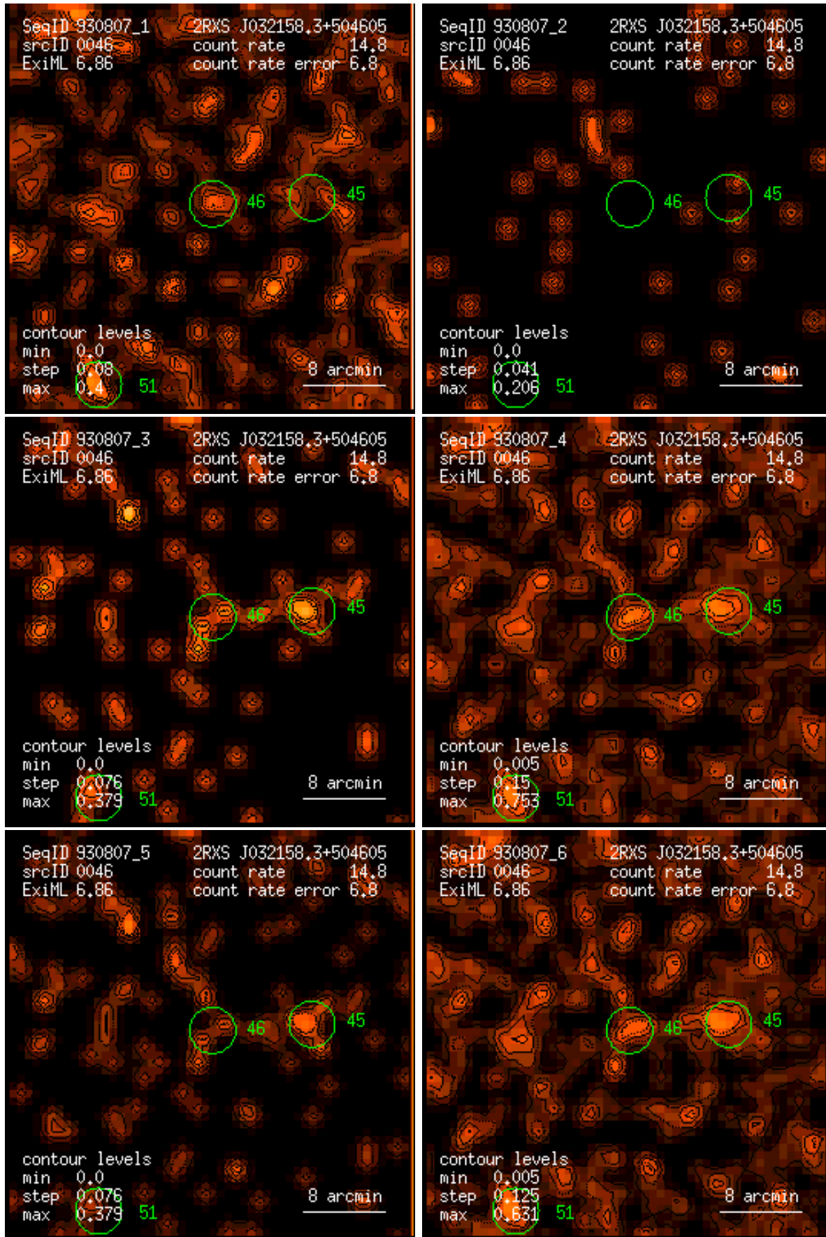
Figure 46: RASS 930807: detection 0046: band rate images, Gaussian filter: (1) PSPC channels 11 – 41, (2) 52 – 90, (3) 91 – 201, (4) 11 – 235, (5) 52 – 201, (6) 11 – 201. Broad band rates in counts/ks. Band rate contour levels in counts/ks/arcmin 2 .
