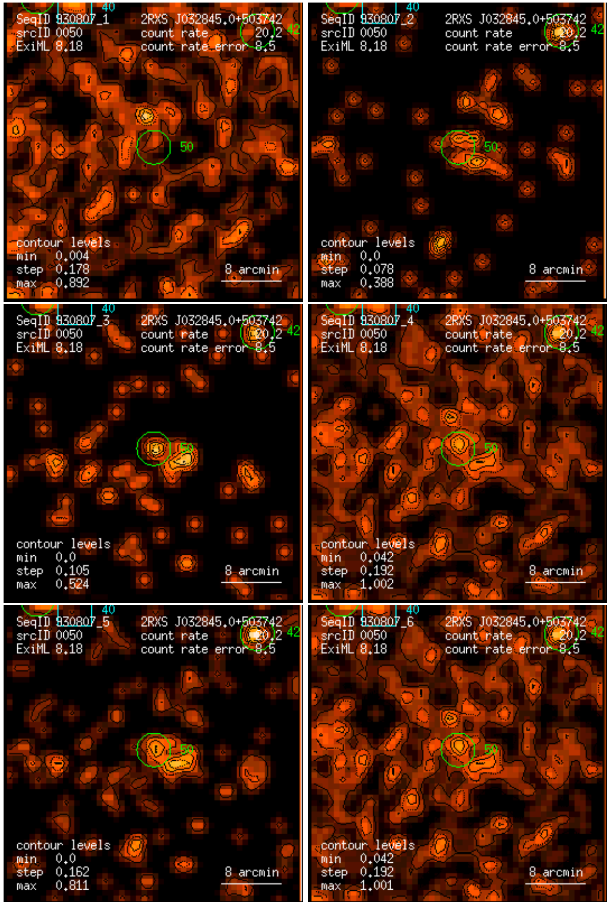
Figure 50: RASS 930807: detection 0050: band rate images, Gaussian filter: (1) PSPC channels 11 – 41, (2) 52 – 90, (3) 91 – 201, (4) 11 – 235, (5) 52 – 201, (6) 11 – 201. Broad band rates in counts/ks. Band rate contour levels in counts/ks/arcmin 2 .
