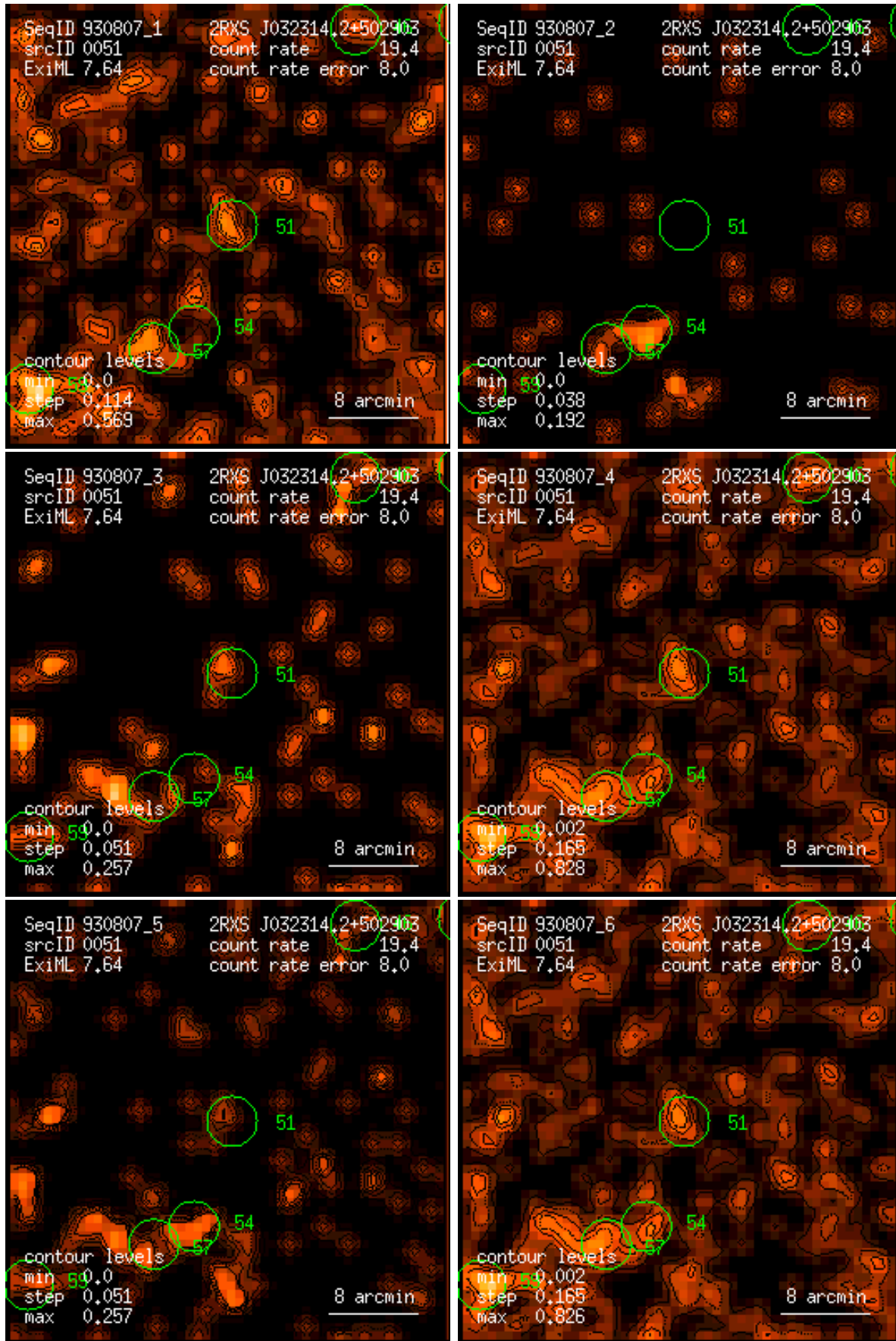
Figure 51: RASS 930807: detection 0051: band rate images, Gaussian filter: (1) PSPC channels 11 – 41, (2) 52 – 90, (3) 91 – 201, (4) 11 – 235, (5) 52 – 201, (6) 11 – 201. Broad band rates in counts/ks. Band rate contour levels in counts/ks/arcmin 2 .
