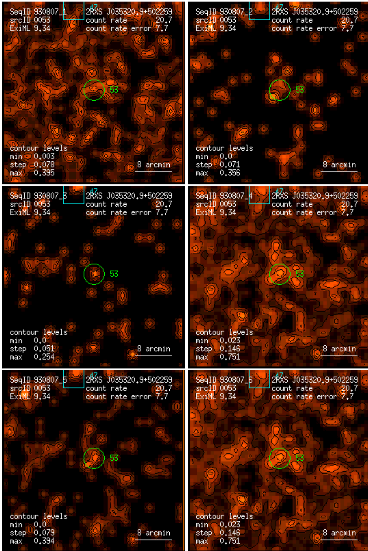
Figure 53: RASS 930807: detection 0053: band rate images, Gaussian filter: (1) PSPC channels 11 – 41, (2) 52 – 90, (3) 91 – 201, (4) 11 – 235, (5) 52 – 201, (6) 11 – 201. Broad band rates in counts/ks. Band rate contour levels in counts/ks/arcmin 2 .
