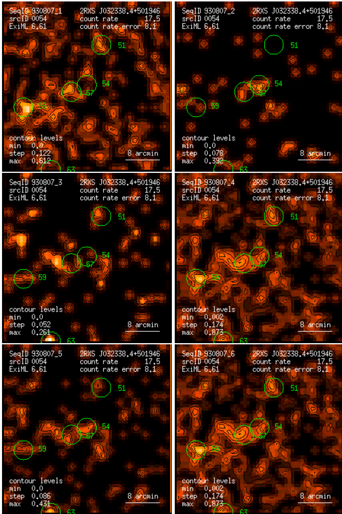
Figure 54: RASS 930807: detection 0054: band rate images, Gaussian filter: (1) PSPC channels 11 – 41, (2) 52 – 90, (3) 91 – 201, (4) 11 – 235, (5) 52 – 201, (6) 11 – 201. Broad band rates in counts/ks. Band rate contour levels in counts/ks/arcmin 2 .
