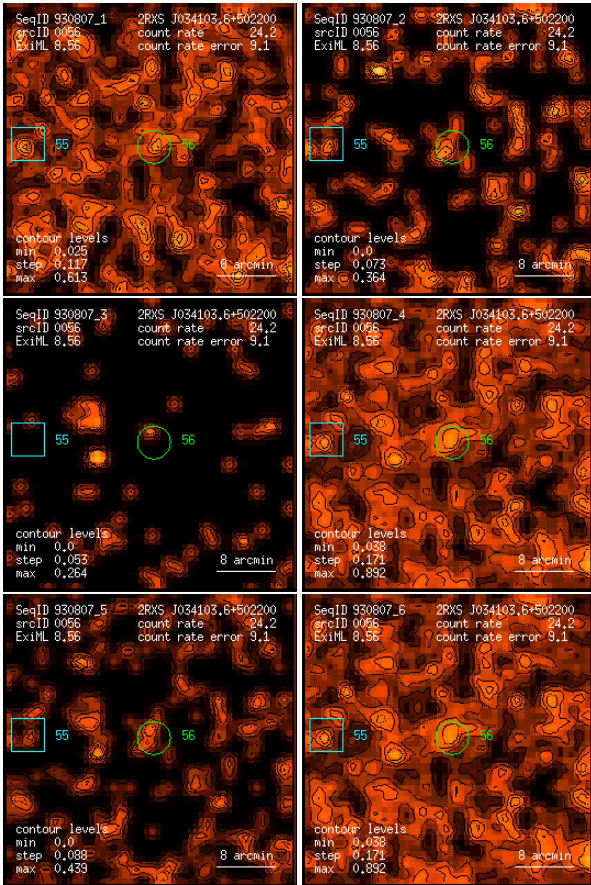
Figure 56: RASS 930807: detection 0056: band rate images, Gaussian filter: (1) PSPC channels 11 – 41, (2) 52 – 90, (3) 91 – 201, (4) 11 – 235, (5) 52 – 201, (6) 11 – 201. Broad band rates in counts/ks. Band rate contour levels in counts/ks/arcmin 2 .
