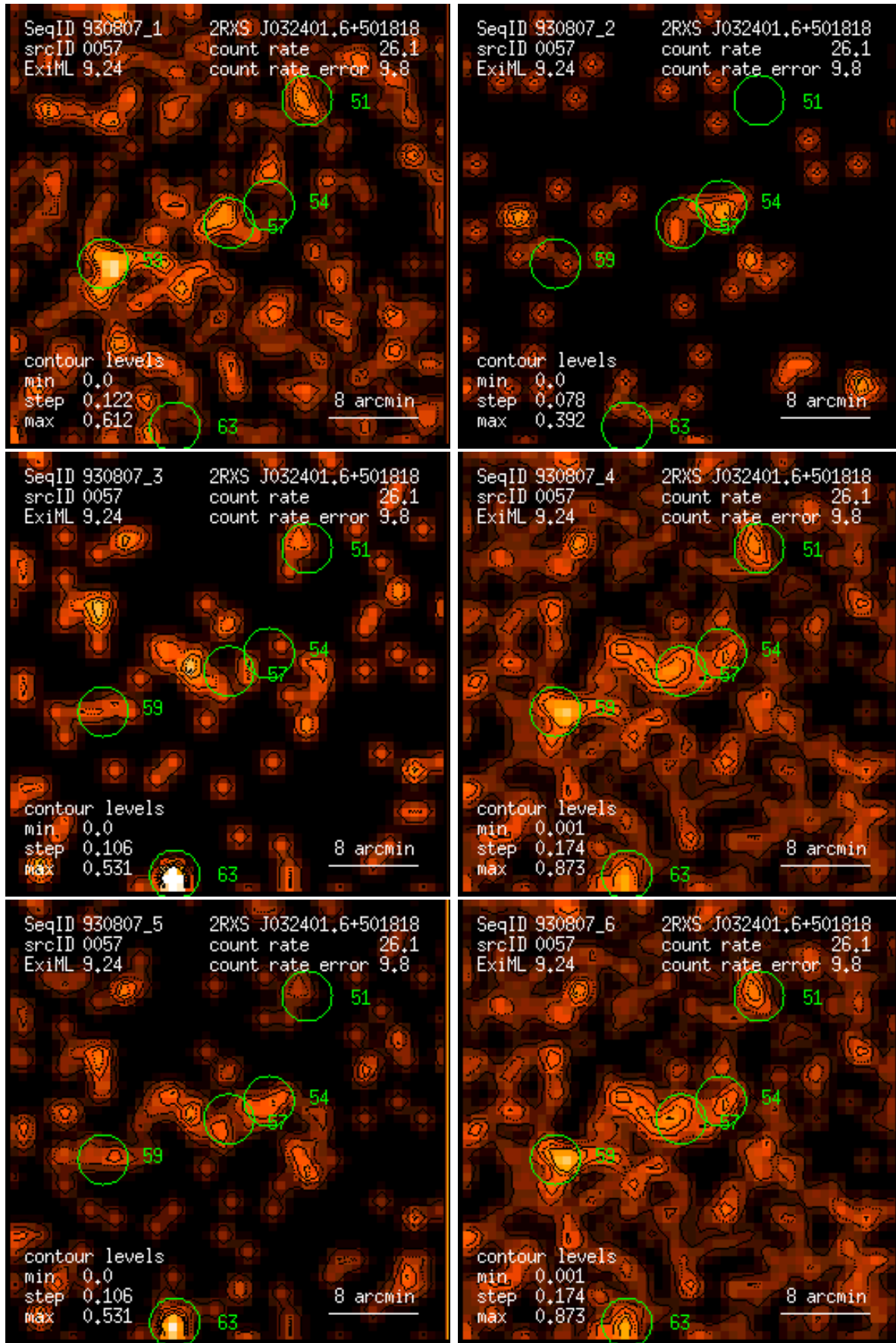
Figure 57: RASS 930807: detection 0057: band rate images, Gaussian filter: (1) PSPC channels 11 – 41, (2) 52 – 90, (3) 91 – 201, (4) 11 – 235, (5) 52 – 201, (6) 11 – 201. Broad band rates in counts/ks. Band rate contour levels in counts/ks/arcmin 2 .
