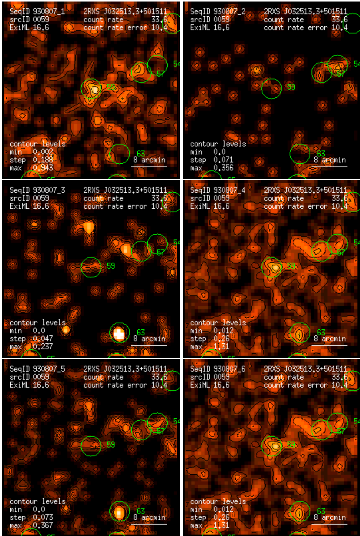
Figure 59: RASS 930807: detection 0059: band rate images, Gaussian filter: (1) PSPC channels 11 – 41, (2) 52 – 90, (3) 91 – 201, (4) 11 – 235, (5) 52 – 201, (6) 11 – 201. Broad band rates in counts/ks. Band rate contour levels in counts/ks/arcmin 2 .
