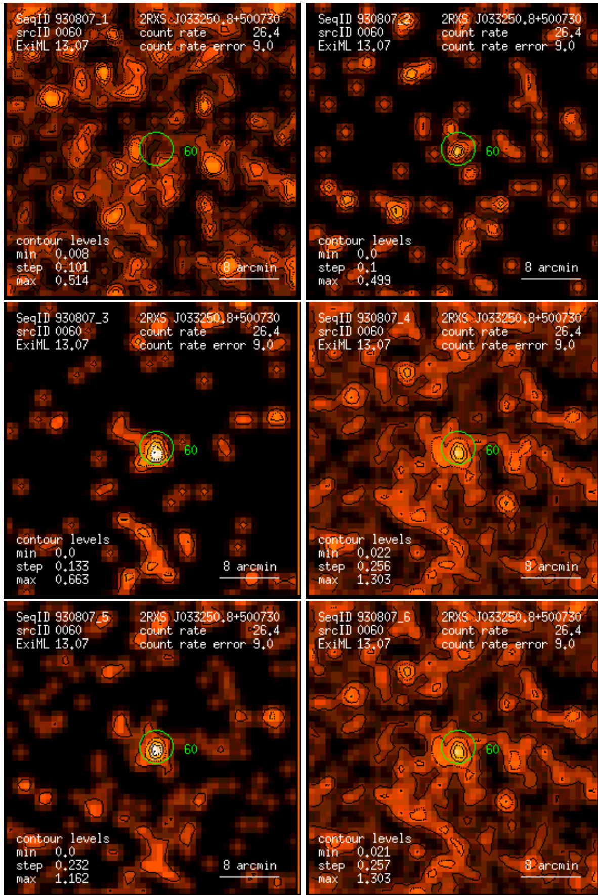
Figure 60: RASS 930807: detection 0060: band rate images, Gaussian filter: (1) PSPC channels 11 – 41, (2) 52 – 90, (3) 91 – 201, (4) 11 – 235, (5) 52 – 201, (6) 11 – 201. Broad band rates in counts/ks. Band rate contour levels in counts/ks/arcmin 2 .
