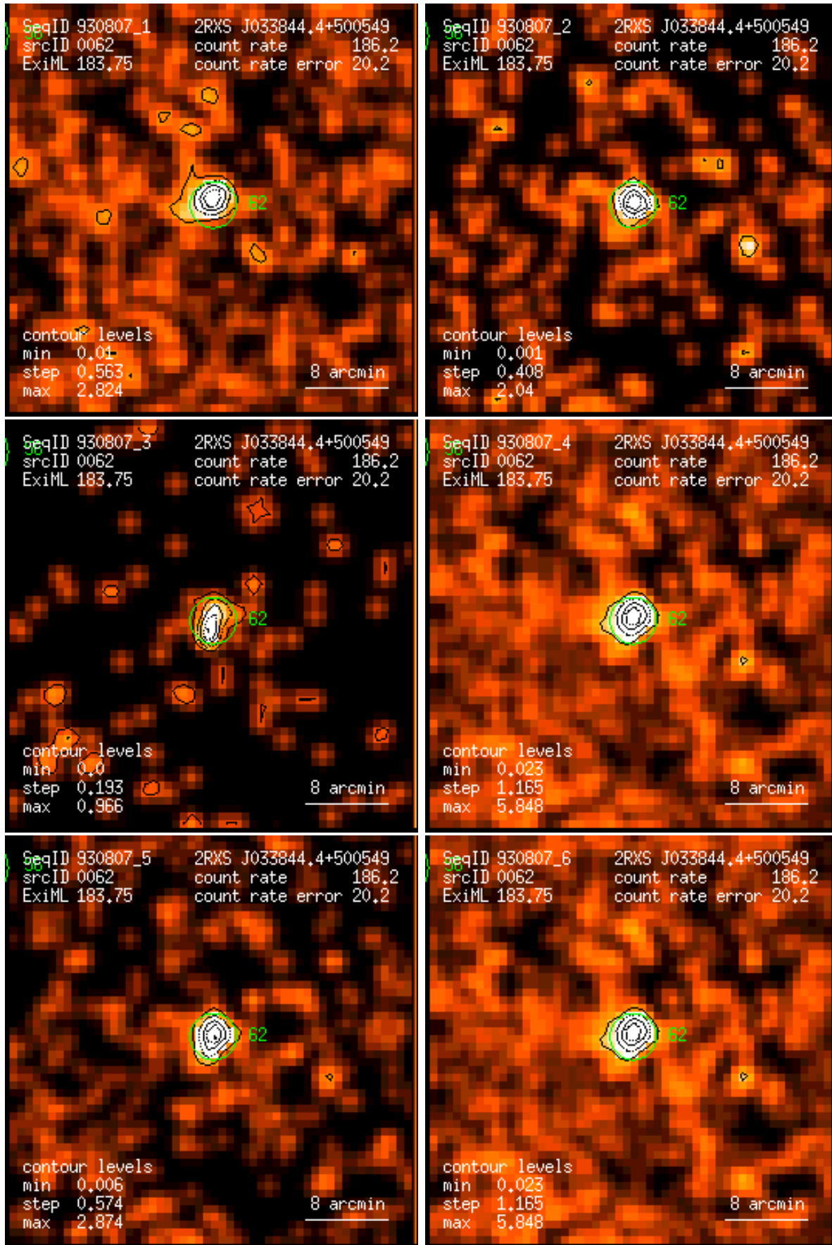
Figure 62: RASS 930807: detection 0062: band rate images, Gaussian filter: (1) PSPC channels 11 – 41, (2) 52 – 90, (3) 91 – 201, (4) 11 – 235, (5) 52 – 201, (6) 11 – 201. Broad band rates in counts/ks. Band rate contour levels in counts/ks/arcmin 2 .
