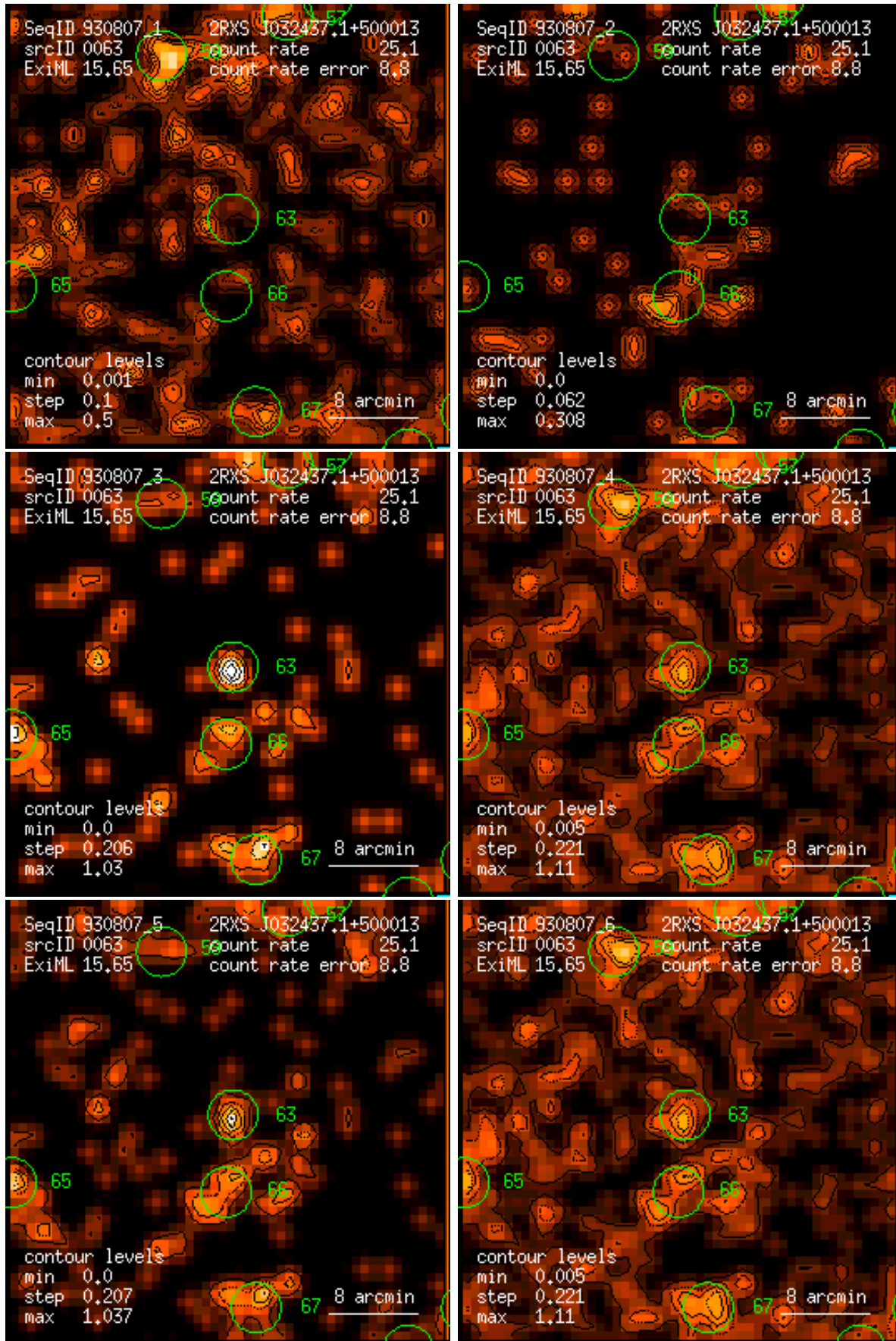
Figure 63: RASS 930807: detection 0063: band rate images, Gaussian filter: (1) PSPC channels 11 – 41, (2) 52 – 90, (3) 91 – 201, (4) 11 – 235, (5) 52 – 201, (6) 11 – 201. Broad band rates in counts/ks. Band rate contour levels in counts/ks/arcmin 2 .
