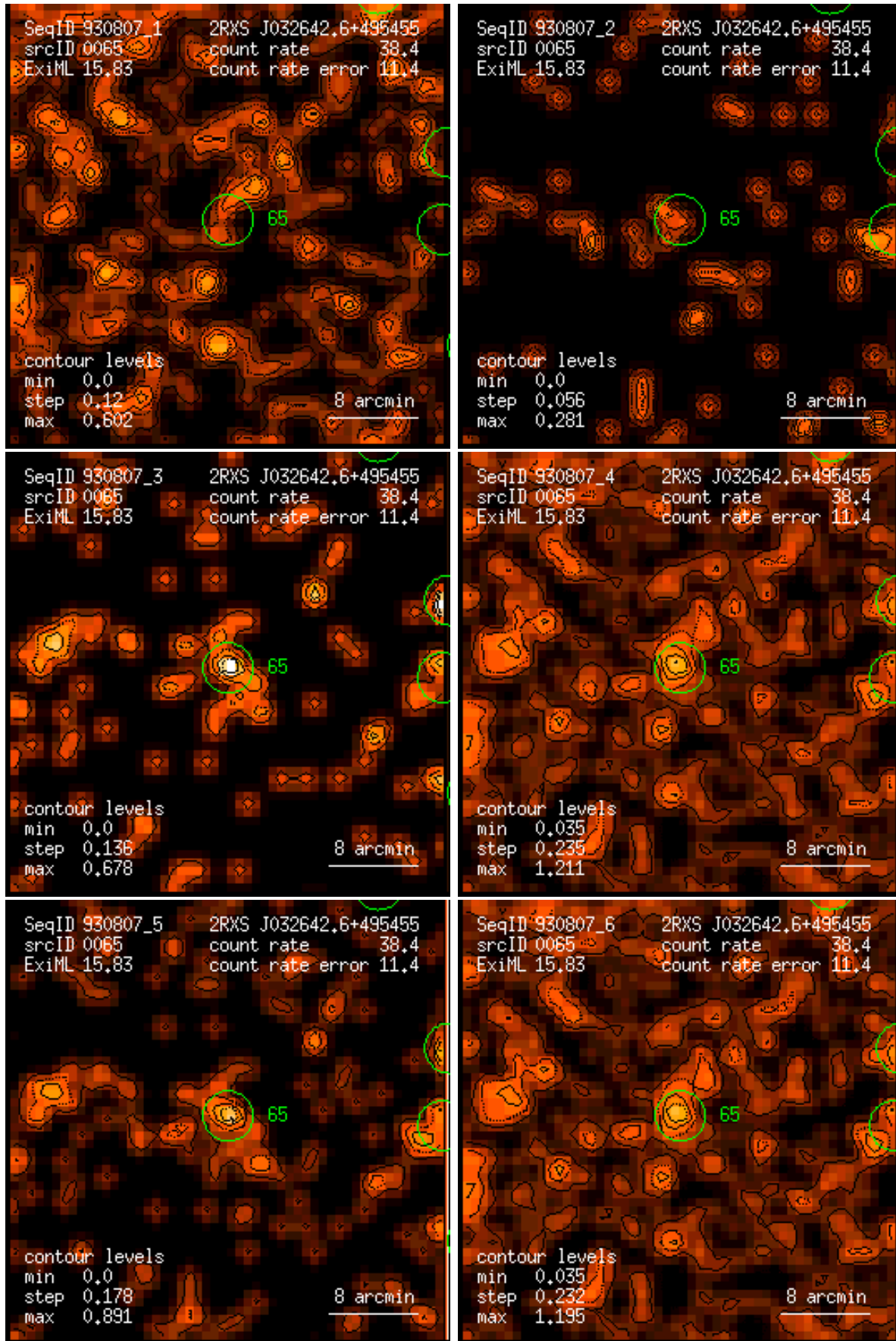
Figure 65: RASS 930807: detection 0065: band rate images, Gaussian filter: (1) PSPC channels 11 – 41, (2) 52 – 90, (3) 91 – 201, (4) 11 – 235, (5) 52 – 201, (6) 11 – 201. Broad band rates in counts/ks. Band rate contour levels in counts/ks/arcmin 2 .
