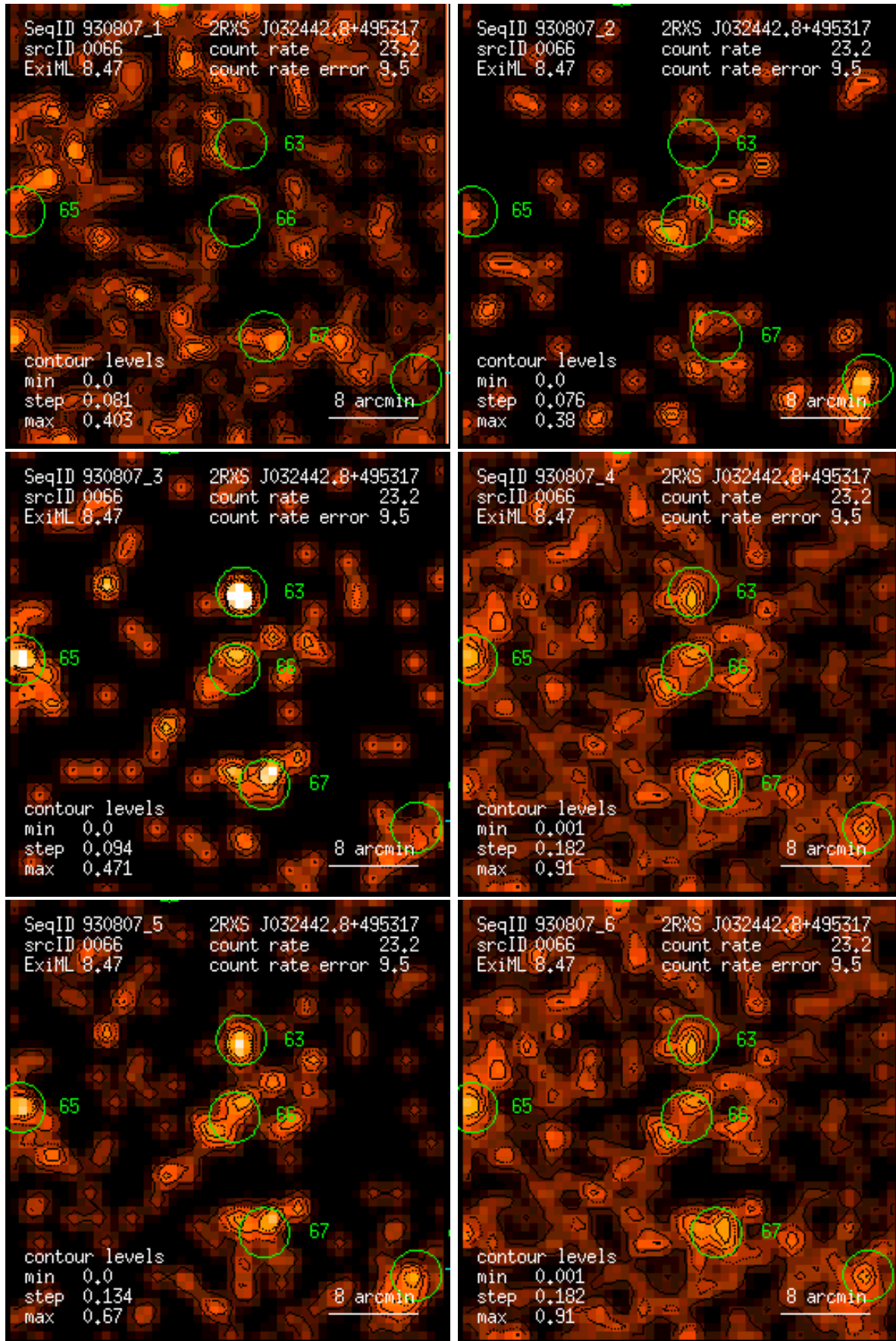
Figure 66: RASS 930807: detection 0066: band rate images, Gaussian filter: (1) PSPC channels 11 – 41, (2) 52 – 90, (3) 91 – 201, (4) 11 – 235, (5) 52 – 201, (6) 11 – 201. Broad band rates in counts/ks. Band rate contour levels in counts/ks/arcmin 2 .
