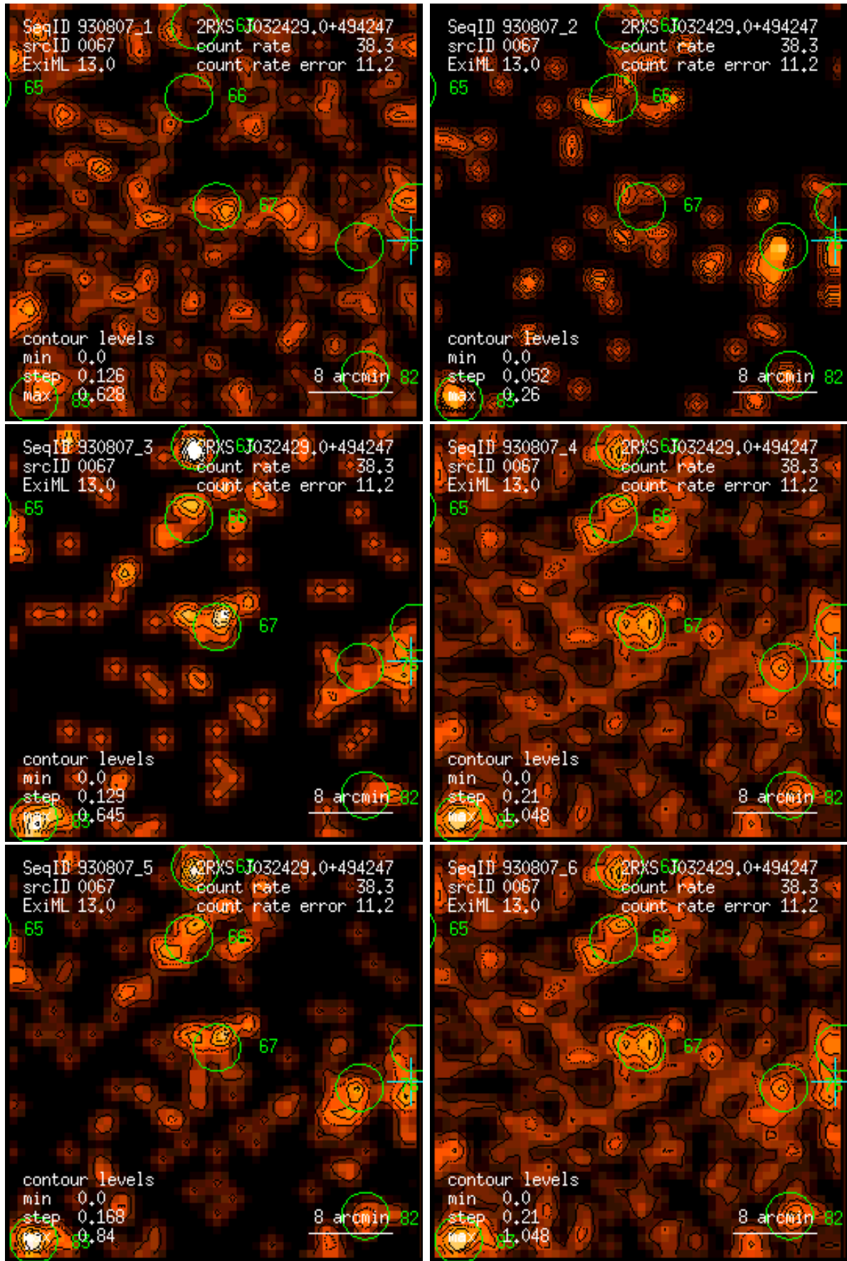
Figure 67: RASS 930807: detection 0067: band rate images, Gaussian filter: (1) PSPC channels 11 – 41, (2) 52 – 90, (3) 91 – 201, (4) 11 – 235, (5) 52 – 201, (6) 11 – 201. Broad band rates in counts/ks. Band rate contour levels in counts/ks/arcmin 2 .
