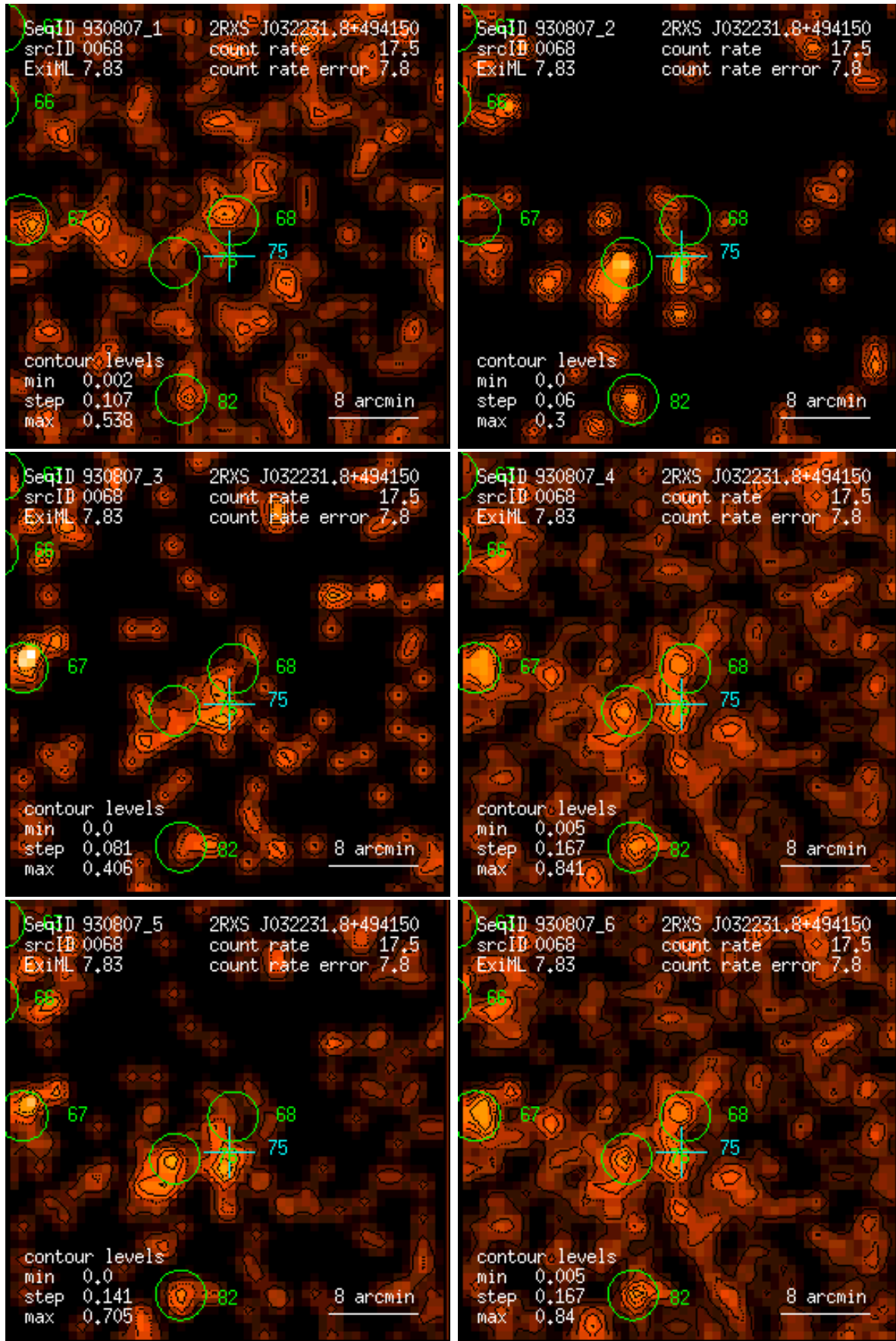
Figure 68: RASS 930807: detection 0068: band rate images, Gaussian filter: (1) PSPC channels 11 – 41, (2) 52 – 90, (3) 91 – 201, (4) 11 – 235, (5) 52 – 201, (6) 11 – 201. Broad band rates in counts/ks. Band rate contour levels in counts/ks/arcmin 2 .
