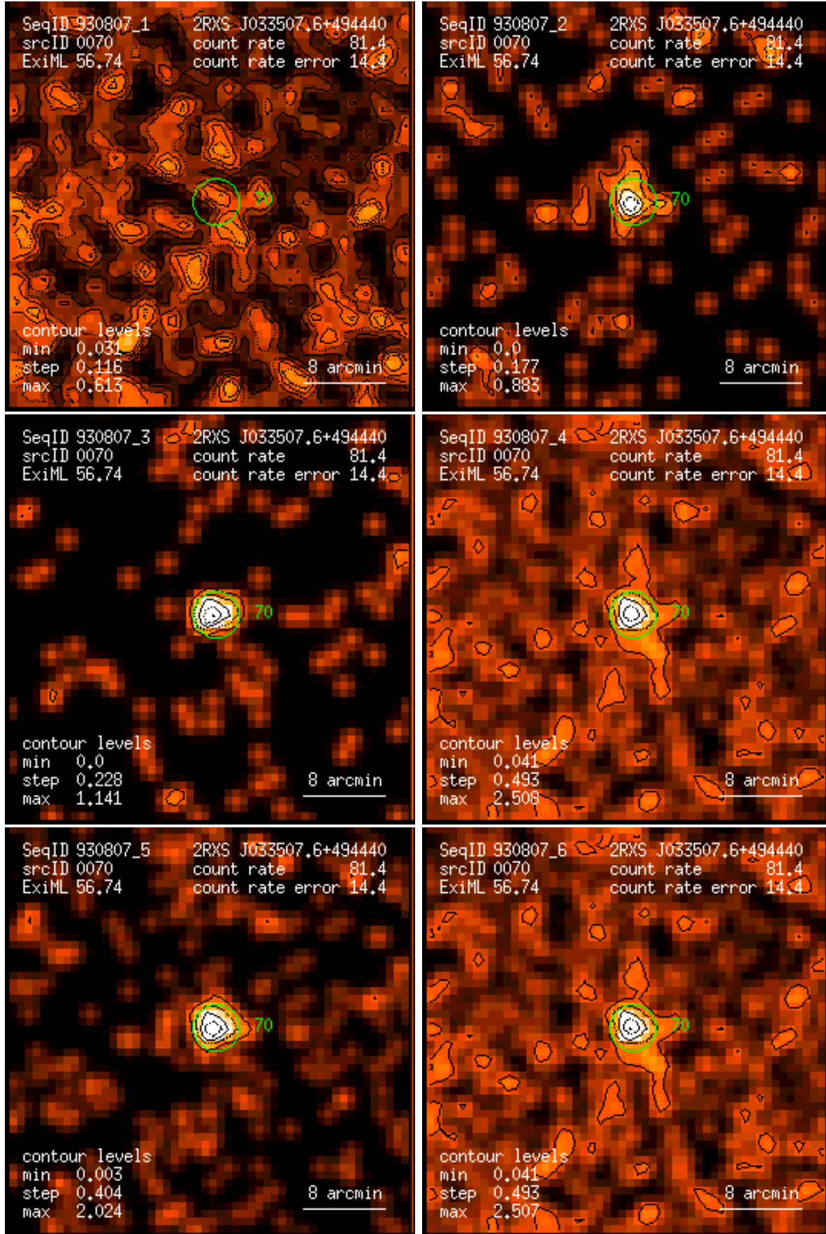
Figure 70: RASS 930807: detection 0070: band rate images, Gaussian filter: (1) PSPC channels 11 – 41, (2) 52 – 90, (3) 91 – 201, (4) 11 – 235, (5) 52 – 201, (6) 11 – 201. Broad band rates in counts/ks. Band rate contour levels in counts/ks/arcmin 2 .
