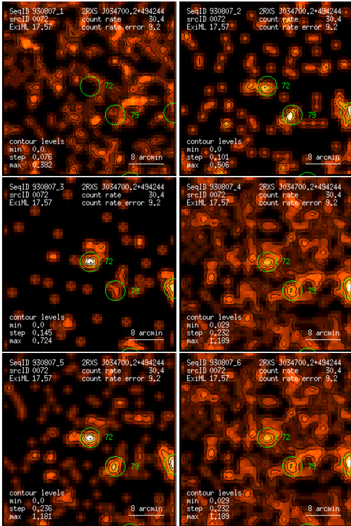
Figure 72: RASS 930807: detection 0072: band rate images, Gaussian filter: (1) PSPC channels 11 – 41, (2) 52 – 90, (3) 91 – 201, (4) 11 – 235, (5) 52 – 201, (6) 11 – 201. Broad band rates in counts/ks. Band rate contour levels in counts/ks/arcmin 2 .
