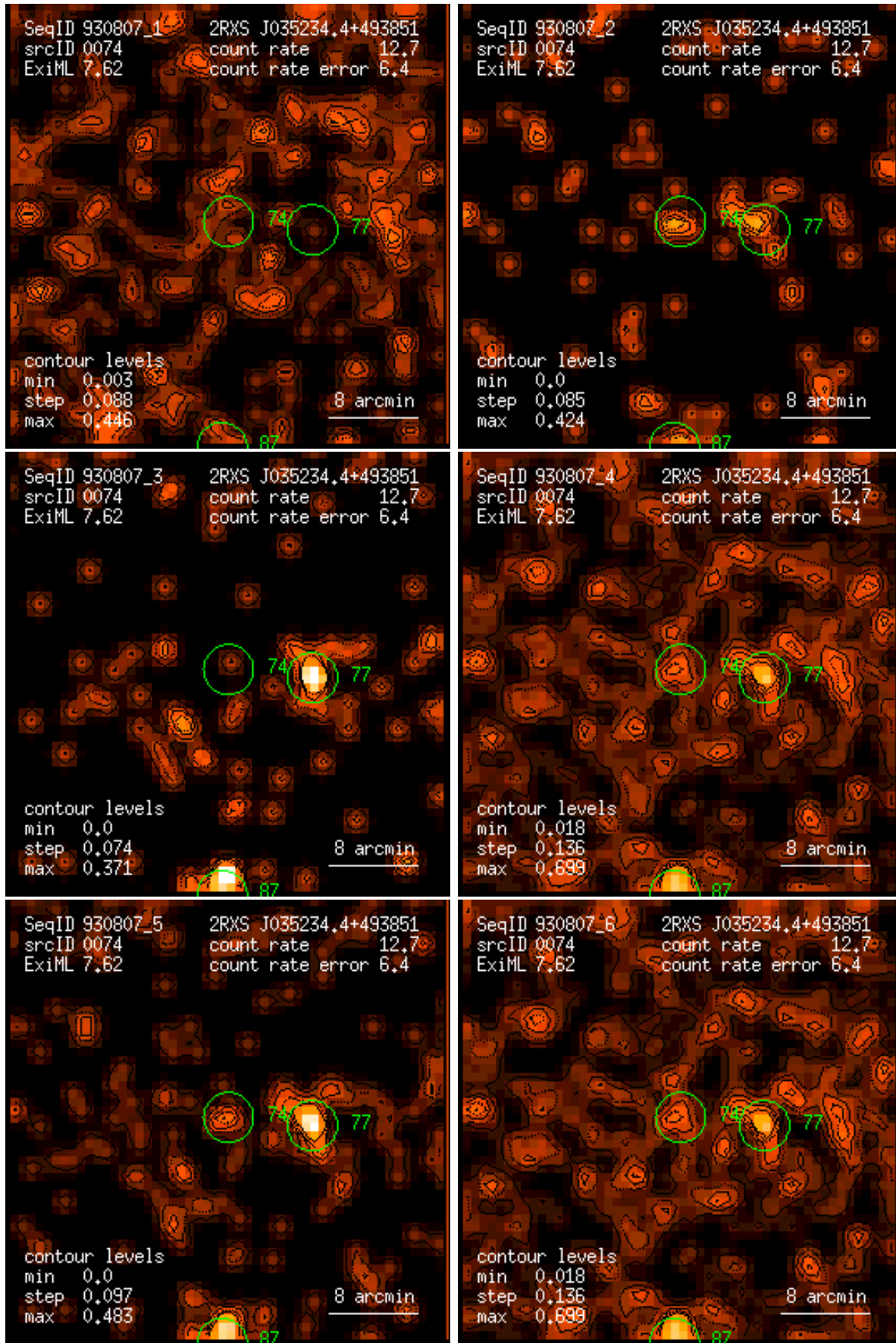
Figure 74: RASS 930807: detection 0074: band rate images, Gaussian filter: (1) PSPC channels 11 – 41, (2) 52 – 90, (3) 91 – 201, (4) 11 – 235, (5) 52 – 201, (6) 11 – 201. Broad band rates in counts/ks. Band rate contour levels in counts/ks/arcmin 2 .
