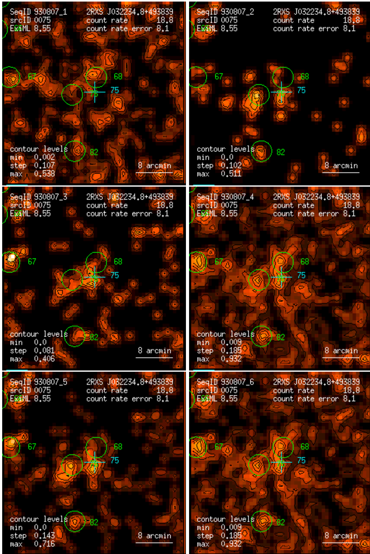
Figure 75: RASS 930807: detection 0075: band rate images, Gaussian filter: (1) PSPC channels 11 – 41, (2) 52 – 90, (3) 91 – 201, (4) 11 – 235, (5) 52 – 201, (6) 11 – 201. Broad band rates in counts/ks. Band rate contour levels in counts/ks/arcmin 2 .
