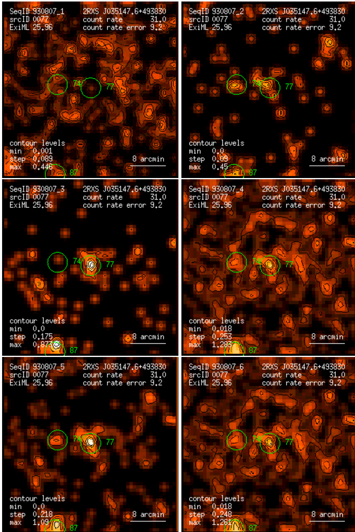
Figure 77: RASS 930807: detection 0077: band rate images, Gaussian filter: (1) PSPC channels 11 – 41, (2) 52 – 90, (3) 91 – 201, (4) 11 – 235, (5) 52 – 201, (6) 11 – 201. Broad band rates in counts/ks. Band rate contour levels in counts/ks/arcmin 2 .
