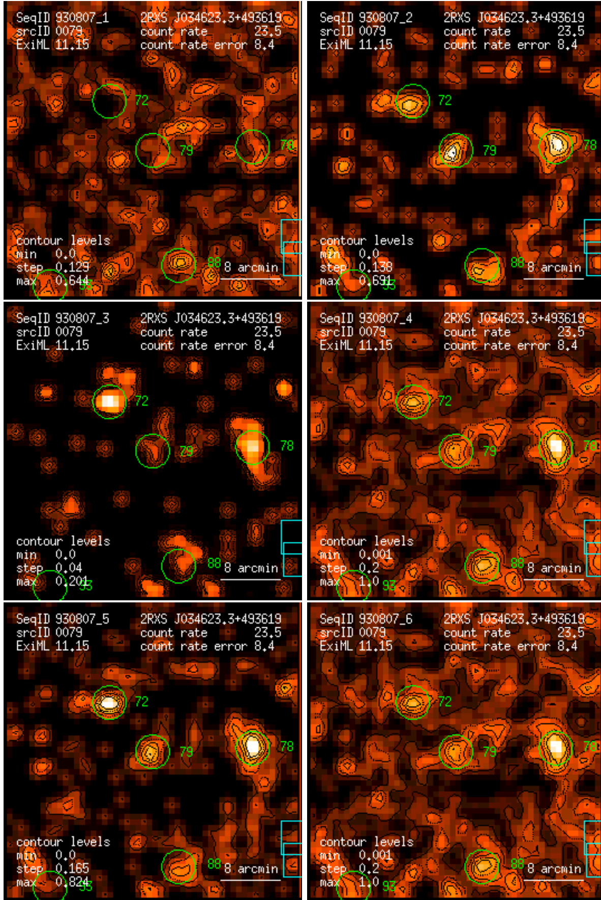
Figure 79: RASS 930807: detection 0079: band rate images, Gaussian filter: (1) PSPC channels 11 – 41, (2) 52 – 90, (3) 91 – 201, (4) 11 – 235, (5) 52 – 201, (6) 11 – 201. Broad band rates in counts/ks. Band rate contour levels in counts/ks/arcmin 2 .
