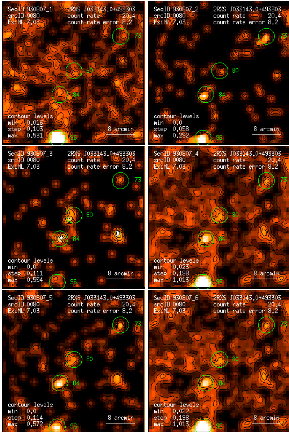
Figure 80: RASS 930807: detection 0080: band rate images, Gaussian filter: (1) PSPC channels 11 – 41, (2) 52 – 90, (3) 91 – 201, (4) 11 – 235, (5) 52 – 201, (6) 11 – 201. Broad band rates in counts/ks. Band rate contour levels in counts/ks/arcmin 2 .
