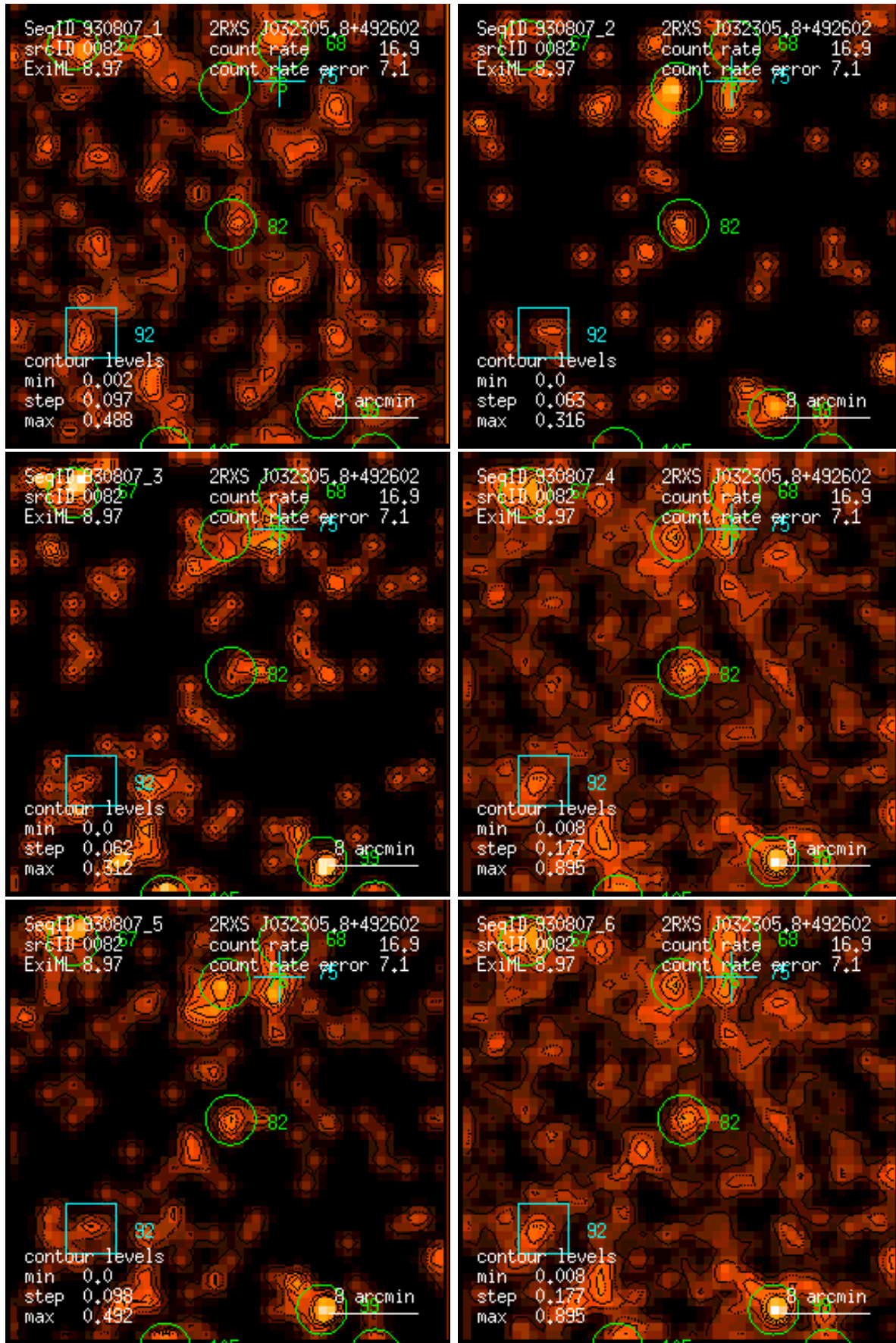
Figure 82: RASS 930807: detection 0082: band rate images, Gaussian filter: (1) PSPC channels 11 – 41, (2) 52 – 90, (3) 91 – 201, (4) 11 – 235, (5) 52 – 201, (6) 11 – 201. Broad band rates in counts/ks. Band rate contour levels in counts/ks/arcmin 2 .
