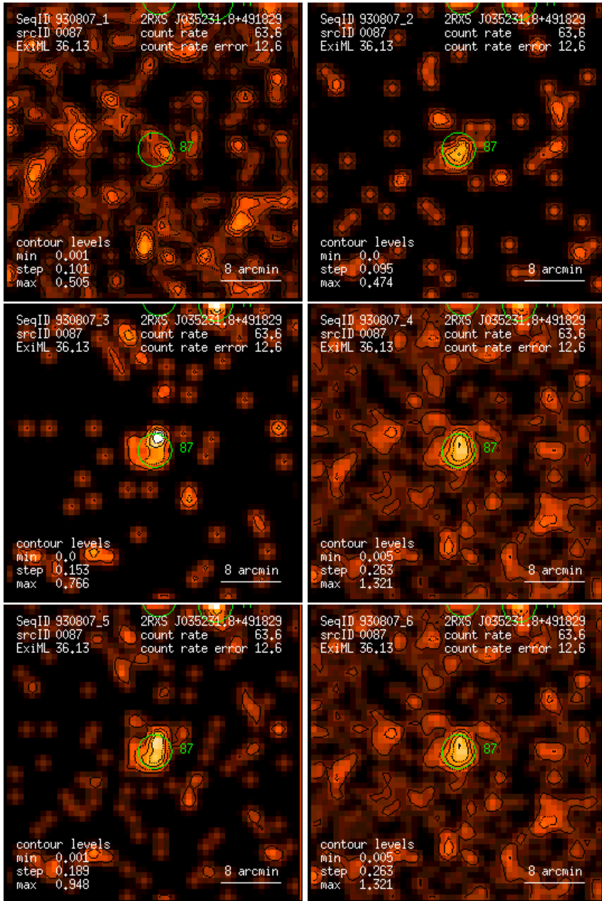
Figure 87: RASS 930807: detection 0087: band rate images, Gaussian filter: (1) PSPC channels 11 – 41, (2) 52 – 90, (3) 91 – 201, (4) 11 – 235, (5) 52 – 201, (6) 11 – 201. Broad band rates in counts/ks. Band rate contour levels in counts/ks/arcmin 2 .
