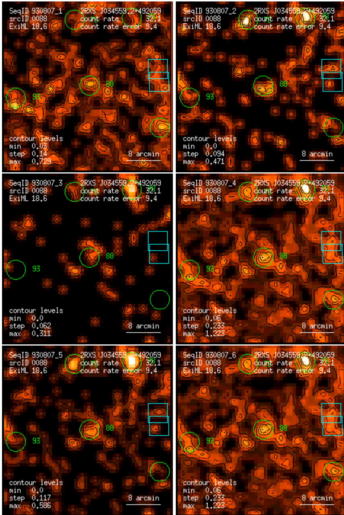
Figure 88: RASS 930807: detection 0088: band rate images, Gaussian filter: (1) PSPC channels 11 – 41, (2) 52 – 90, (3) 91 – 201, (4) 11 – 235, (5) 52 – 201, (6) 11 – 201. Broad band rates in counts/ks. Band rate contour levels in counts/ks/arcmin 2 .
