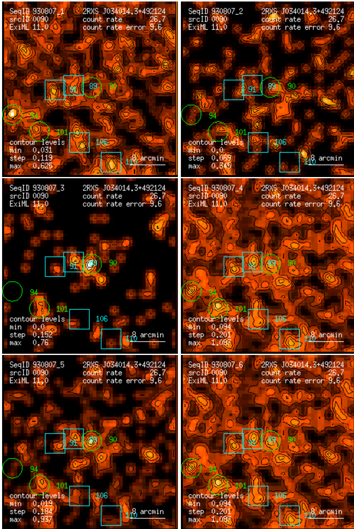
Figure 90: RASS 930807: detection 0090: band rate images, Gaussian filter: (1) PSPC channels 11 – 41, (2) 52 – 90, (3) 91 – 201, (4) 11 – 235, (5) 52 – 201, (6) 11 – 201. Broad band rates in counts/ks. Band rate contour levels in counts/ks/arcmin 2 .
