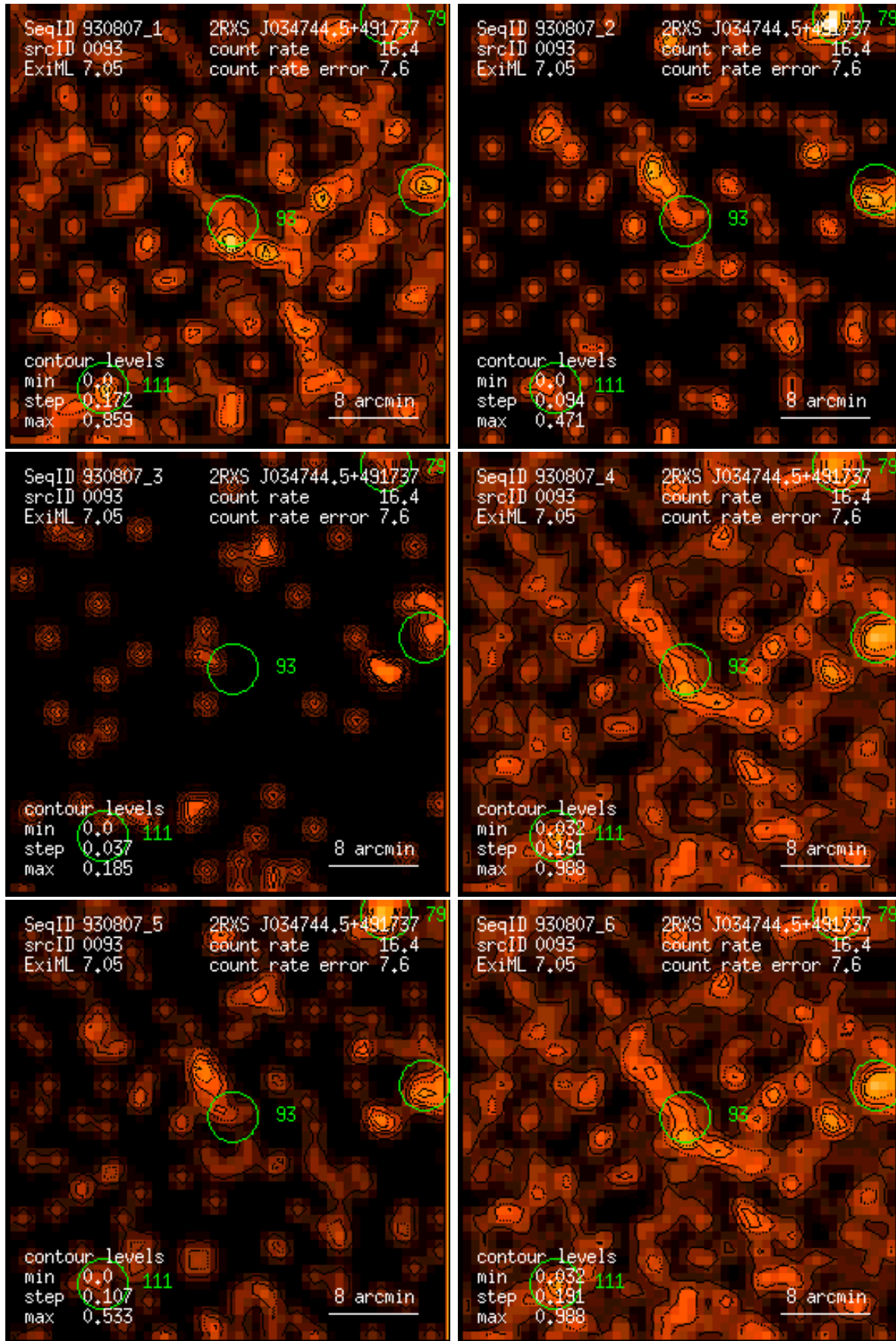
Figure 93: RASS 930807: detection 0093: band rate images, Gaussian filter: (1) PSPC channels 11 – 41, (2) 52 – 90, (3) 91 – 201, (4) 11 – 235, (5) 52 – 201, (6) 11 – 201. Broad band rates in counts/ks. Band rate contour levels in counts/ks/arcmin 2 .
