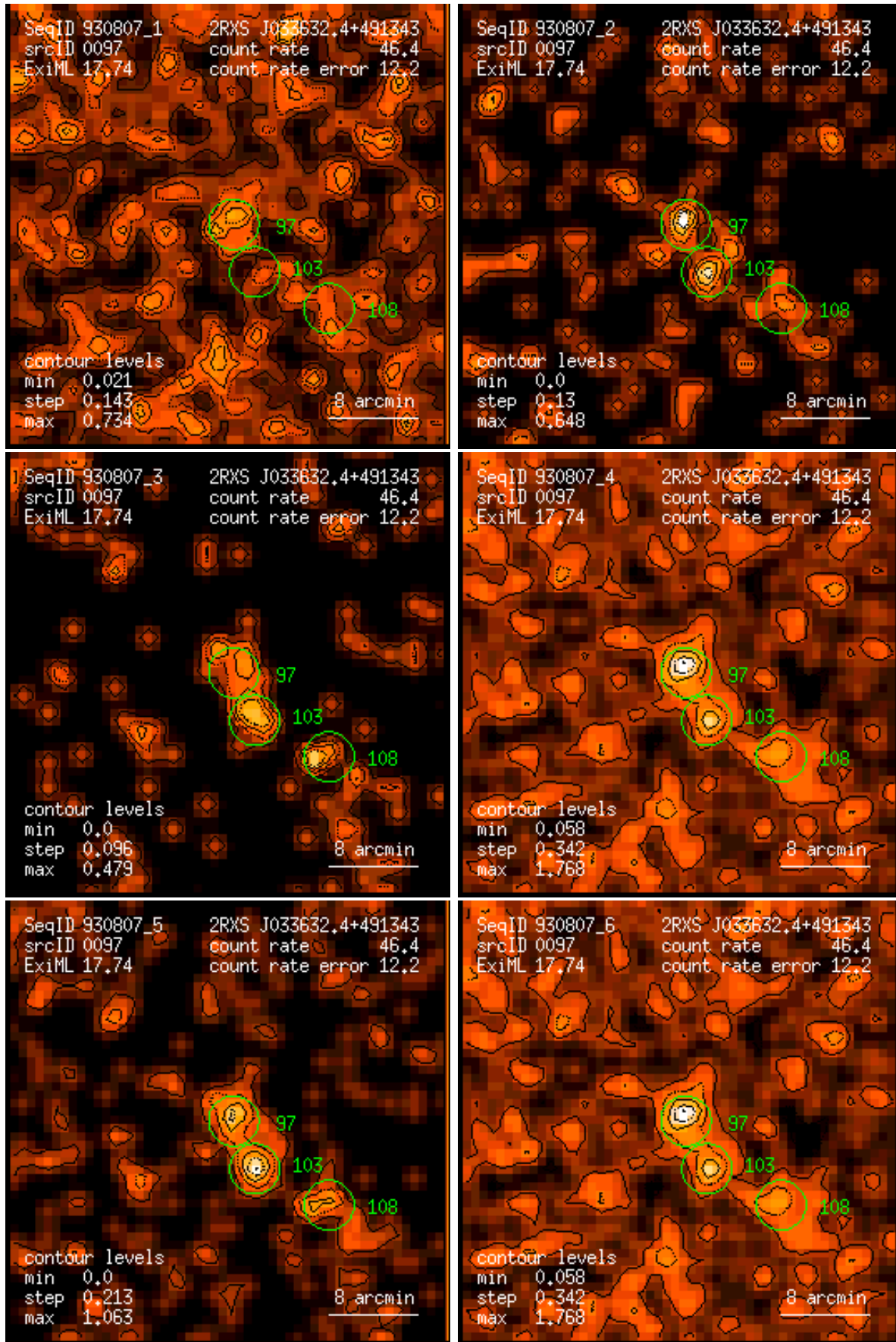
Figure 97: RASS 930807: detection 0097: band rate images, Gaussian filter: (1) PSPC channels 11 – 41, (2) 52 – 90, (3) 91 – 201, (4) 11 – 235, (5) 52 – 201, (6) 11 – 201. Broad band rates in counts/ks. Band rate contour levels in counts/ks/arcmin 2 .
