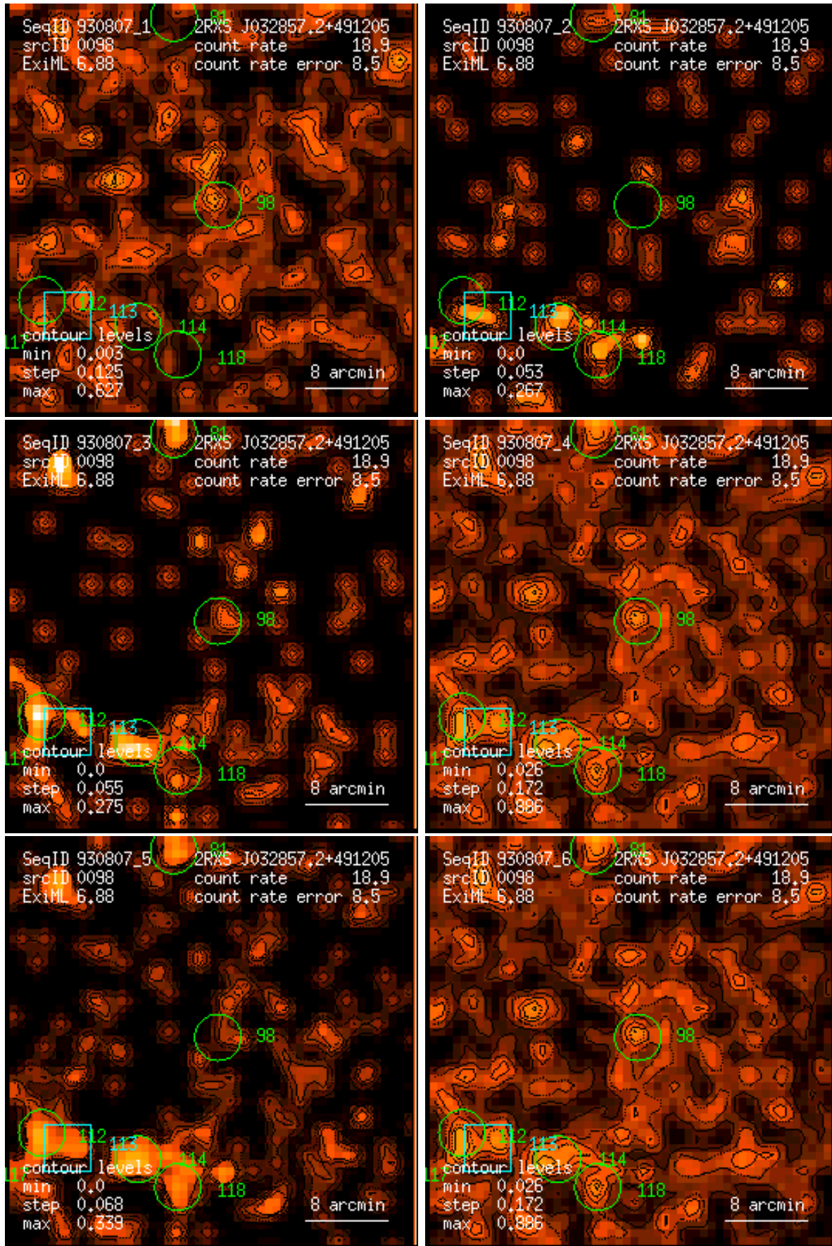
Figure 98: RASS 930807: detection 0098: band rate images, Gaussian filter: (1) PSPC channels 11 – 41, (2) 52 – 90, (3) 91 – 201, (4) 11 – 235, (5) 52 – 201, (6) 11 – 201. Broad band rates in counts/ks. Band rate contour levels in counts/ks/arcmin 2 .
