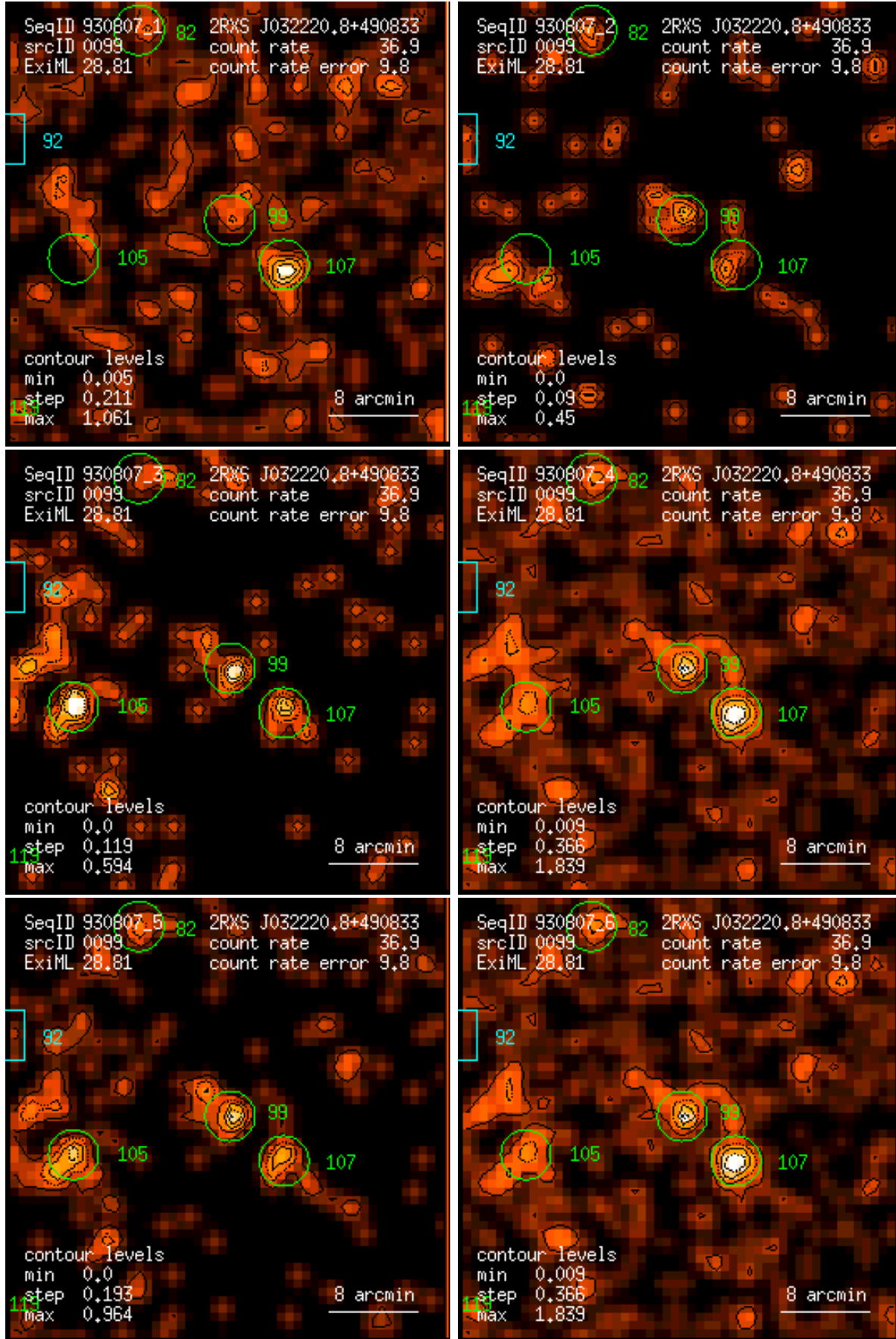
Figure 99: RASS 930807: detection 0099: band rate images, Gaussian filter: (1) PSPC channels 11 – 41, (2) 52 – 90, (3) 91 – 201, (4) 11 – 235, (5) 52 – 201, (6) 11 – 201. Broad band rates in counts/ks. Band rate contour levels in counts/ks/arcmin 2 .
