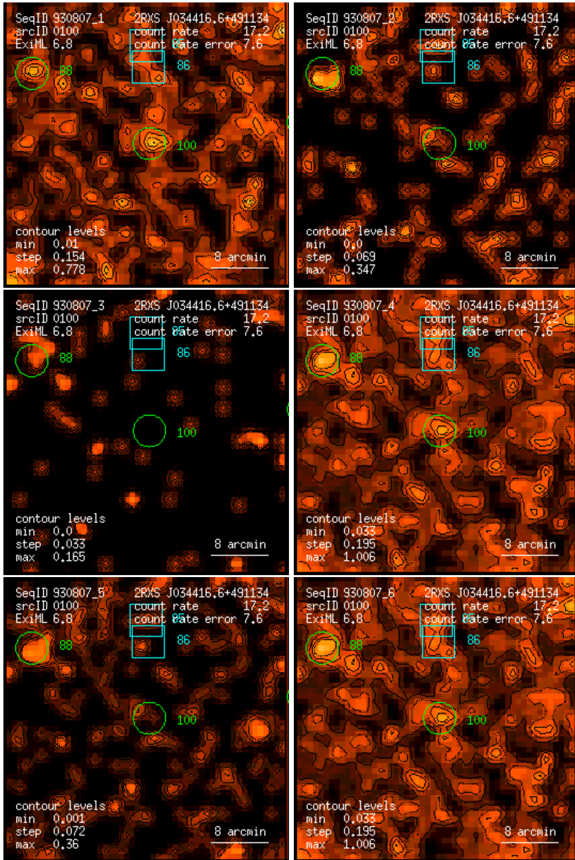
Figure 100: RASS 930807: detection 0100: band rate images, Gaussian filter: (1) PSPC channels 11 – 41, (2) 52 – 90, (3) 91 – 201, (4) 11 – 235, (5) 52 – 201, (6) 11 – 201. Broad band rates in counts/ks. Band rate contour levels in counts/ks/arcmin 2 .
