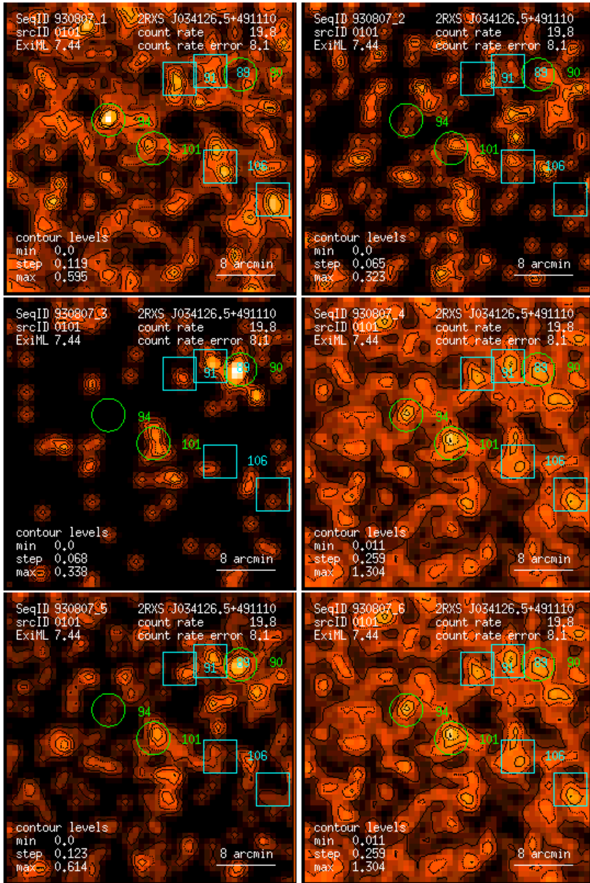
Figure 101: RASS 930807: detection 0101: band rate images, Gaussian filter: (1) PSPC channels 11 – 41, (2) 52 – 90, (3) 91 – 201, (4) 11 – 235, (5) 52 – 201, (6) 11 – 201. Broad band rates in counts/ks. Band rate contour levels in counts/ks/arcmin 2 .
