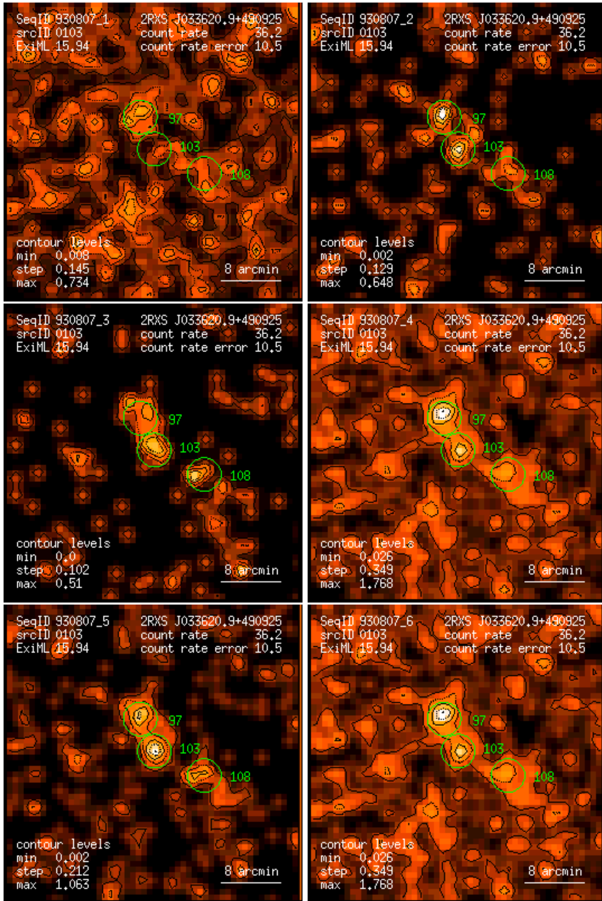
Figure 103: RASS 930807: detection 0103: band rate images, Gaussian filter: (1) PSPC channels 11 – 41, (2) 52 – 90, (3) 91 – 201, (4) 11 – 235, (5) 52 – 201, (6) 11 – 201. Broad band rates in counts/ks. Band rate contour levels in counts/ks/arcmin 2 .
