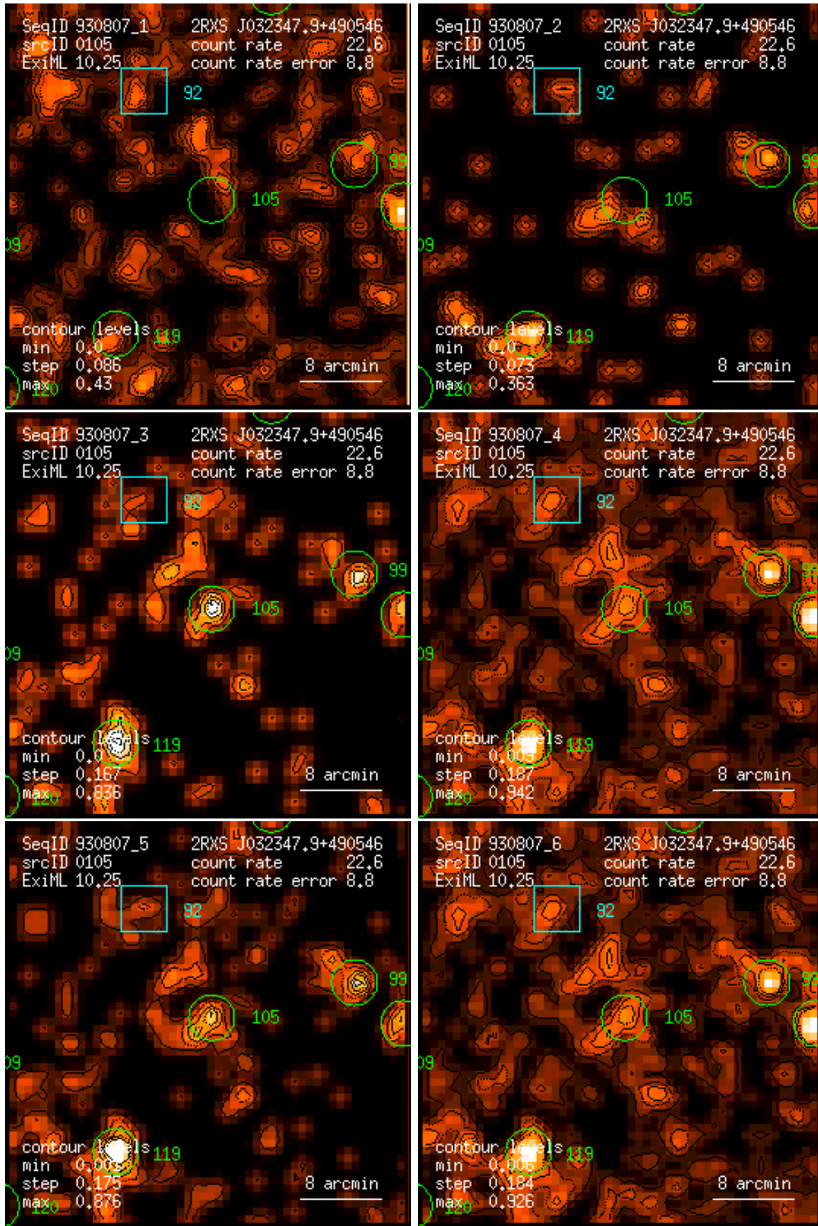
Figure 105: RASS 930807: detection 0105: band rate images, Gaussian filter: (1) PSPC channels 11 – 41, (2) 52 – 90, (3) 91 – 201, (4) 11 – 235, (5) 52 – 201, (6) 11 – 201. Broad band rates in counts/ks. Band rate contour levels in counts/ks/arcmin 2 .
