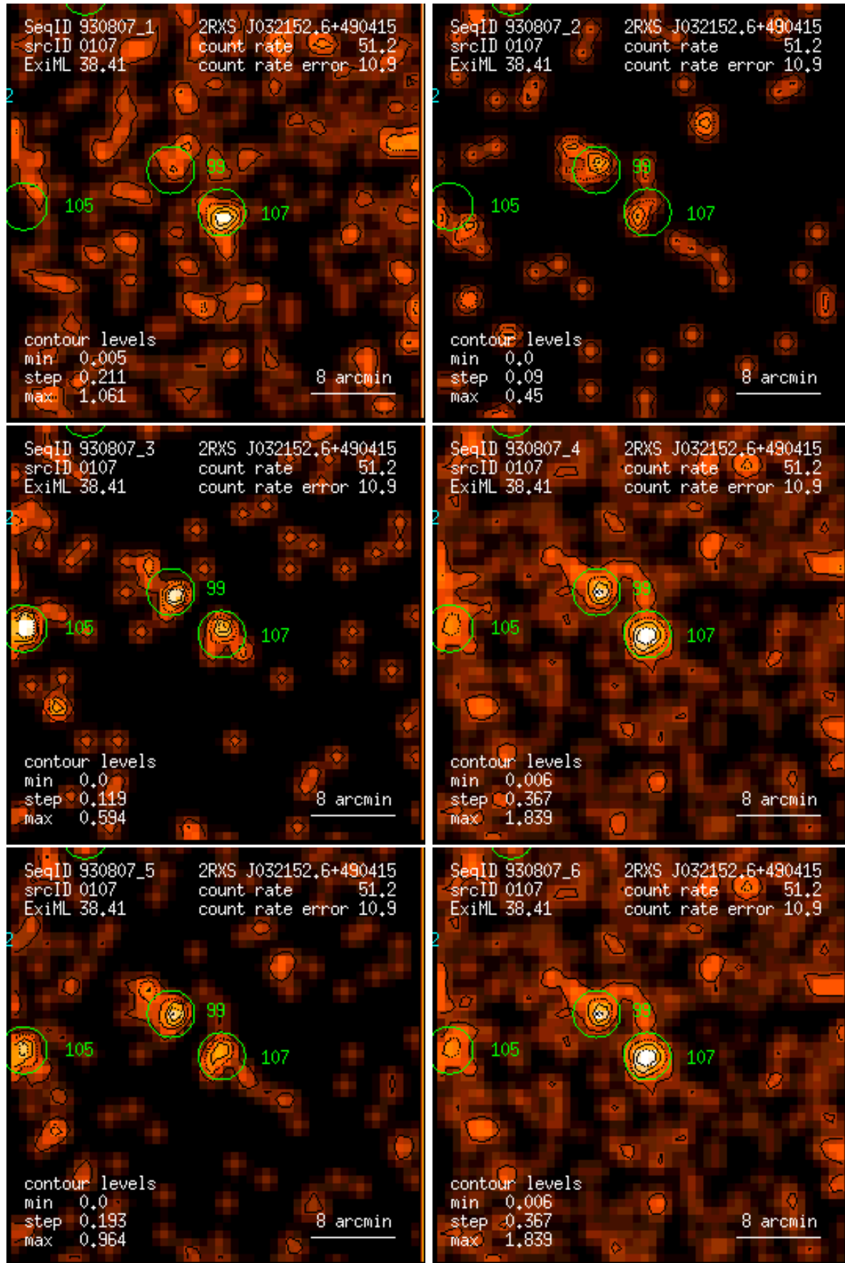
Figure 107: RASS 930807: detection 0107: band rate images, Gaussian filter: (1) PSPC channels 11 – 41, (2) 52 – 90, (3) 91 – 201, (4) 11 – 235, (5) 52 – 201, (6) 11 – 201. Broad band rates in counts/ks. Band rate contour levels in counts/ks/arcmin 2 .
