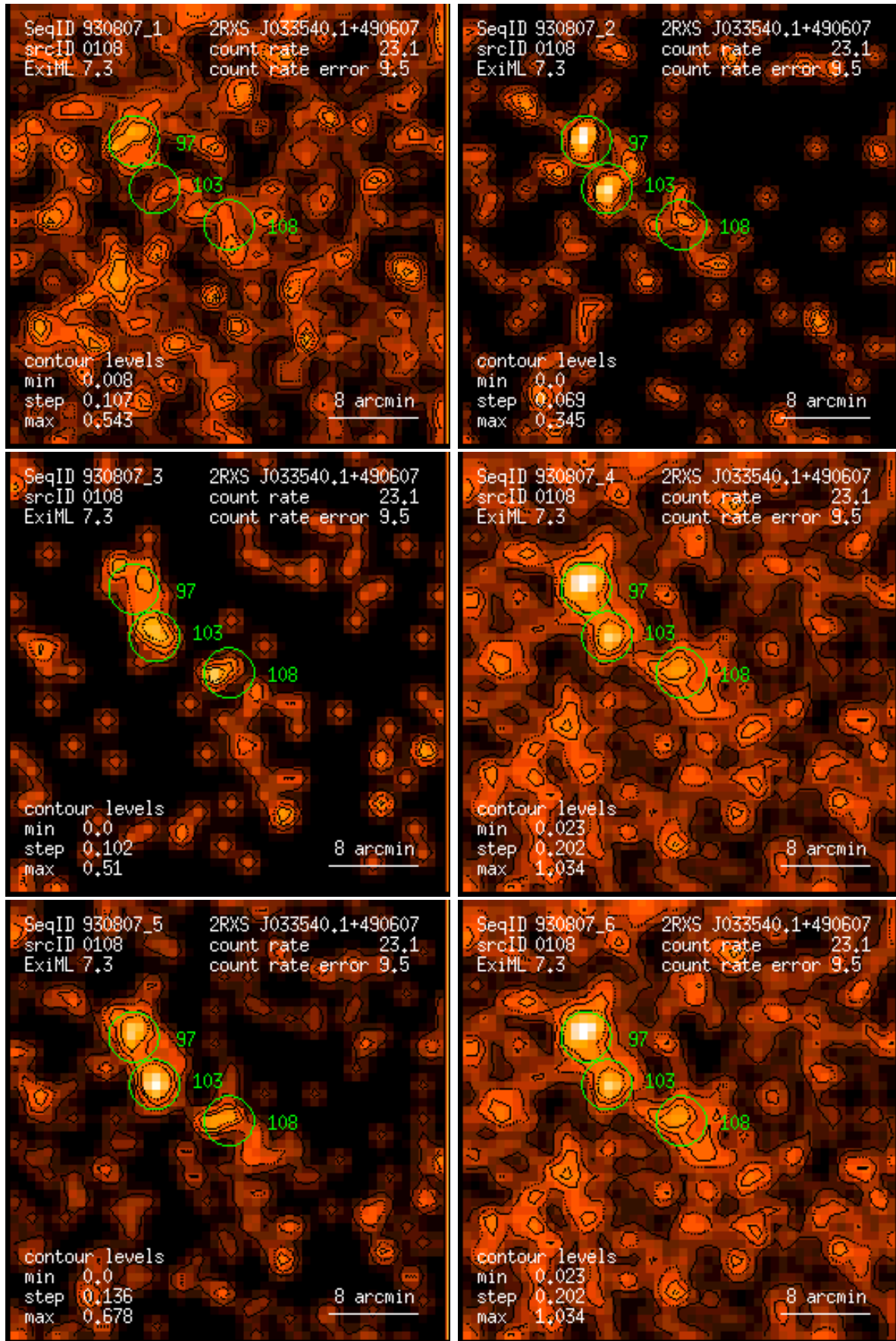
Figure 108: RASS 930807: detection 0108: band rate images, Gaussian filter: (1) PSPC channels 11 – 41, (2) 52 – 90, (3) 91 – 201, (4) 11 – 235, (5) 52 – 201, (6) 11 – 201. Broad band rates in counts/ks. Band rate contour levels in counts/ks/arcmin 2 .
