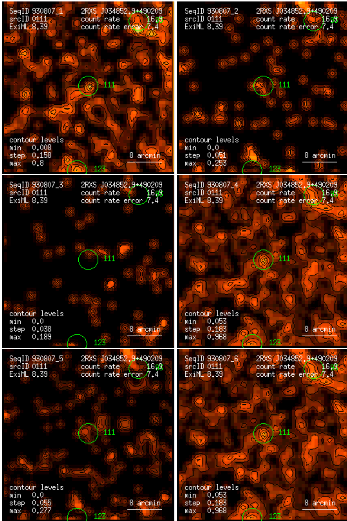
Figure 111: RASS 930807: detection 0111: band rate images, Gaussian filter: (1) PSPC channels 11 – 41, (2) 52 – 90, (3) 91 – 201, (4) 11 – 235, (5) 52 – 201, (6) 11 – 201. Broad band rates in counts/ks. Band rate contour levels in counts/ks/arcmin 2 .
