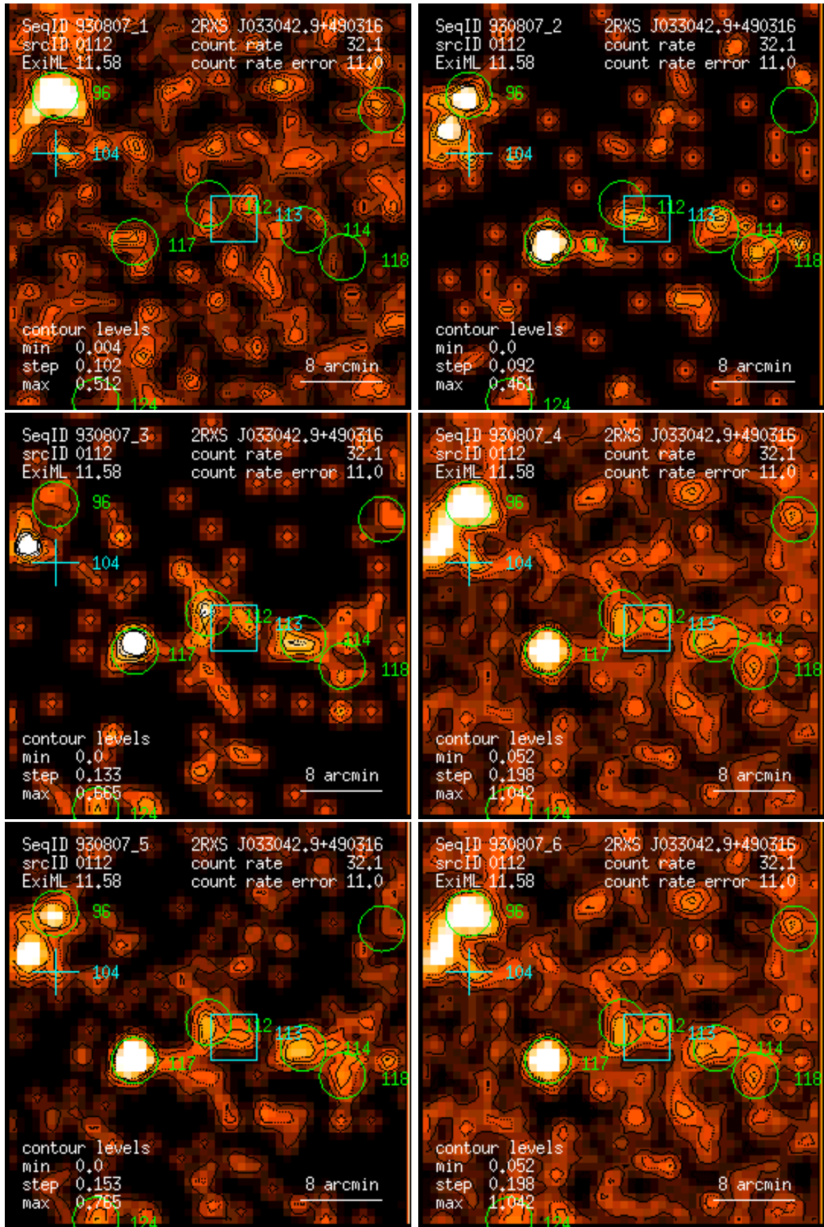
Figure 112: RASS 930807: detection 0112: band rate images, Gaussian filter: (1) PSPC channels 11 – 41, (2) 52 – 90, (3) 91 – 201, (4) 11 – 235, (5) 52 – 201, (6) 11 – 201. Broad band rates in counts/ks. Band rate contour levels in counts/ks/arcmin 2 .
