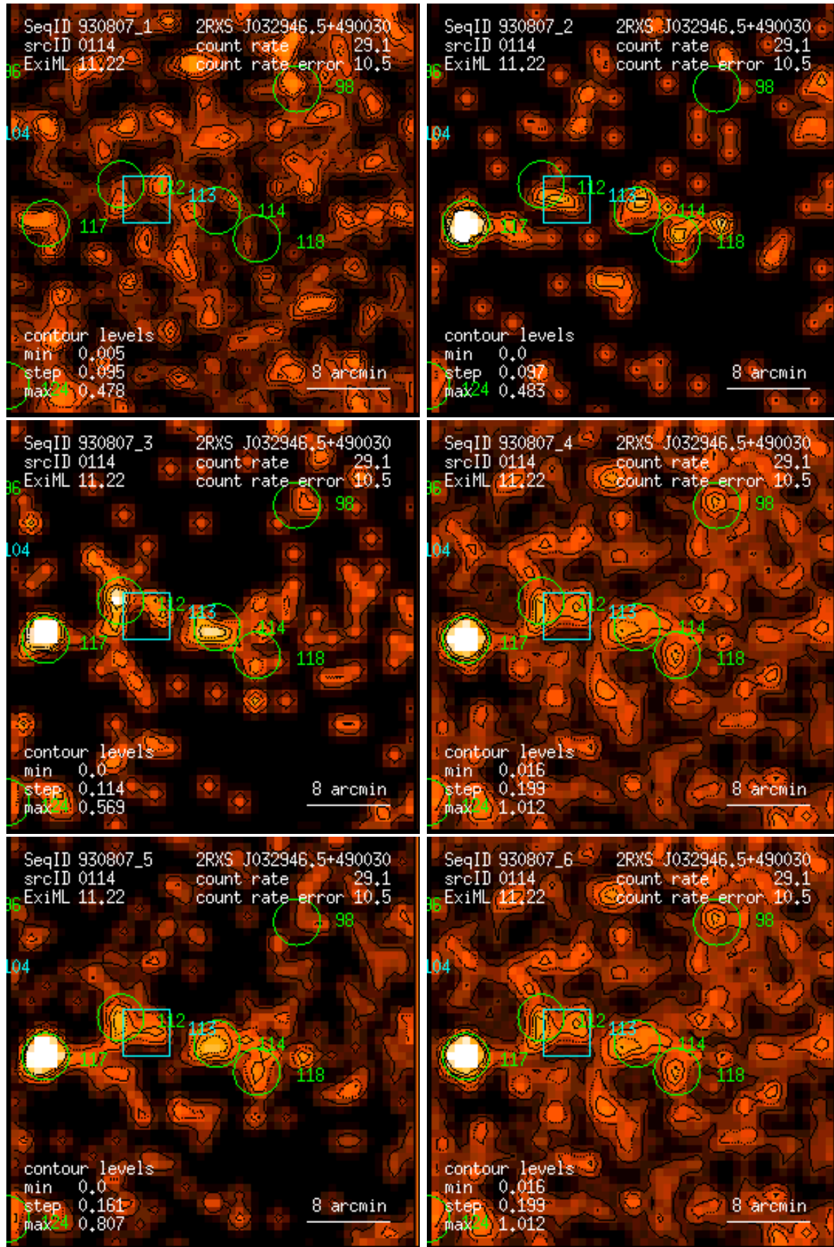
Figure 114: RASS 930807: detection 0114: band rate images, Gaussian filter: (1) PSPC channels 11 – 41, (2) 52 – 90, (3) 91 – 201, (4) 11 – 235, (5) 52 – 201, (6) 11 – 201. Broad band rates in counts/ks. Band rate contour levels in counts/ks/arcmin 2 .
