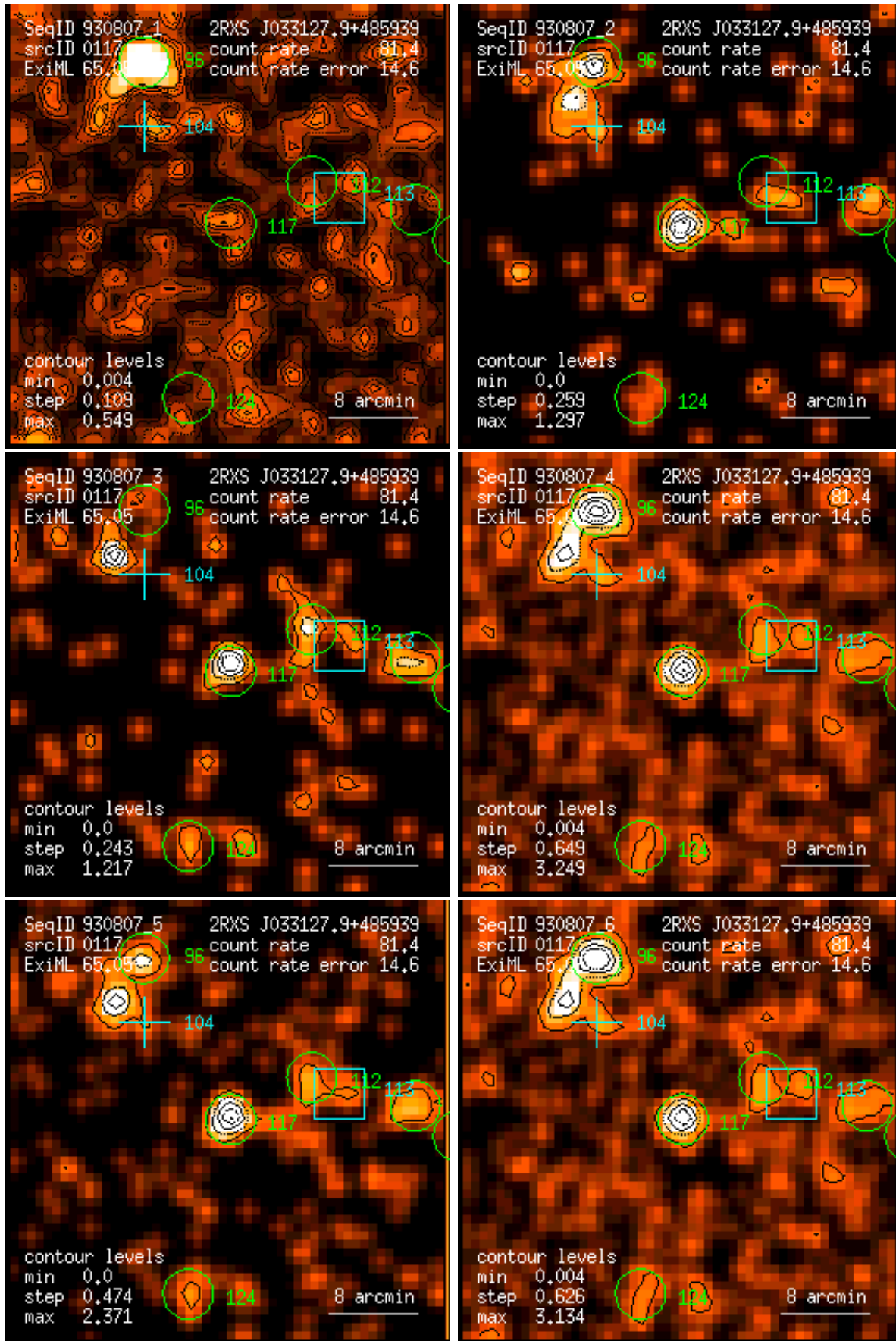
Figure 117: RASS 930807: detection 0117: band rate images, Gaussian filter: (1) PSPC channels 11 – 41, (2) 52 – 90, (3) 91 – 201, (4) 11 – 235, (5) 52 – 201, (6) 11 – 201. Broad band rates in counts/ks. Band rate contour levels in counts/ks/arcmin 2 .
