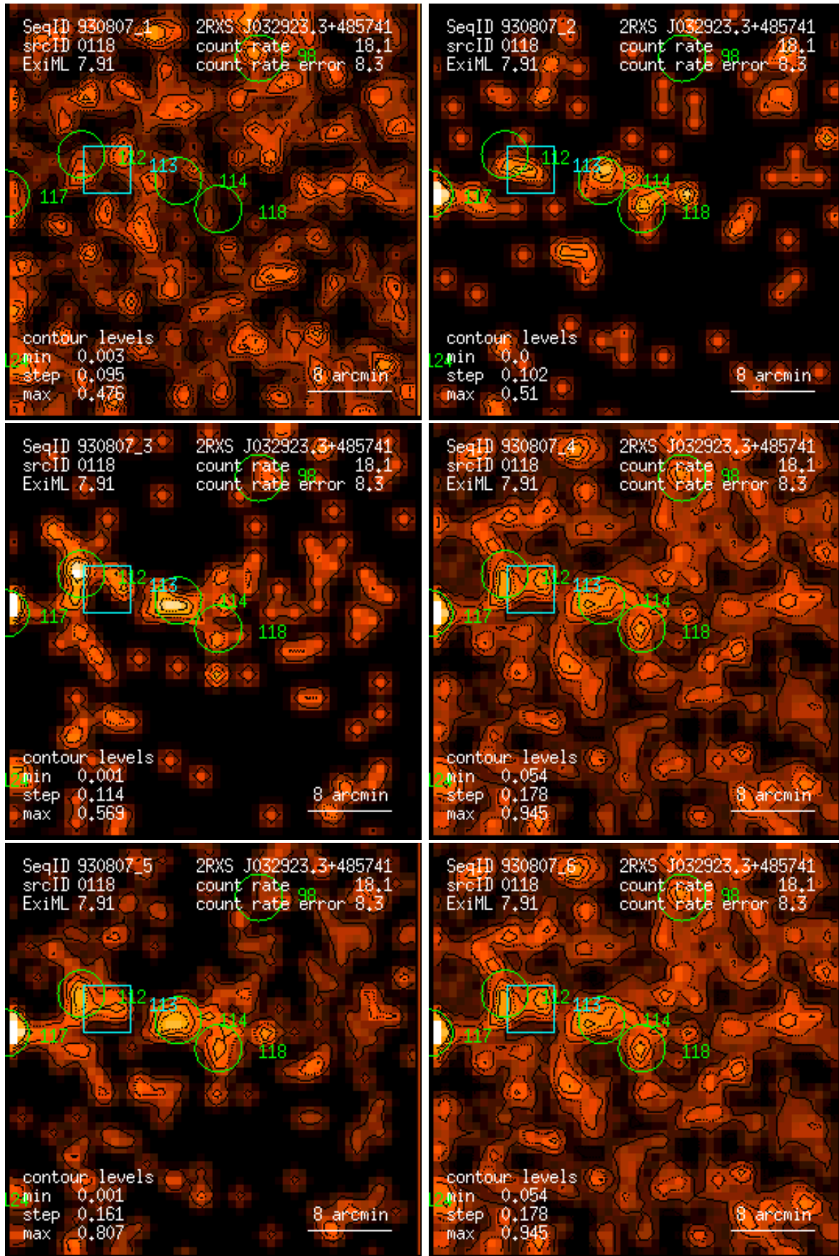
Figure 118: RASS 930807: detection 0118: band rate images, Gaussian filter: (1) PSPC channels 11 – 41, (2) 52 – 90, (3) 91 – 201, (4) 11 – 235, (5) 52 – 201, (6) 11 – 201. Broad band rates in counts/ks. Band rate contour levels in counts/ks/arcmin 2 .
