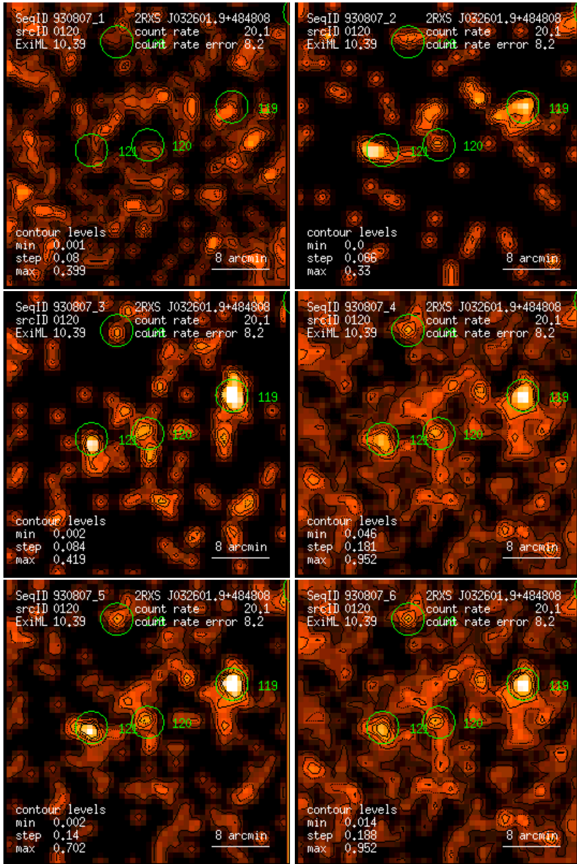
Figure 120: RASS 930807: detection 0120: band rate images, Gaussian filter: (1) PSPC channels 11 – 41, (2) 52 – 90, (3) 91 – 201, (4) 11 – 235, (5) 52 – 201, (6) 11 – 201. Broad band rates in counts/ks. Band rate contour levels in counts/ks/arcmin 2 .
