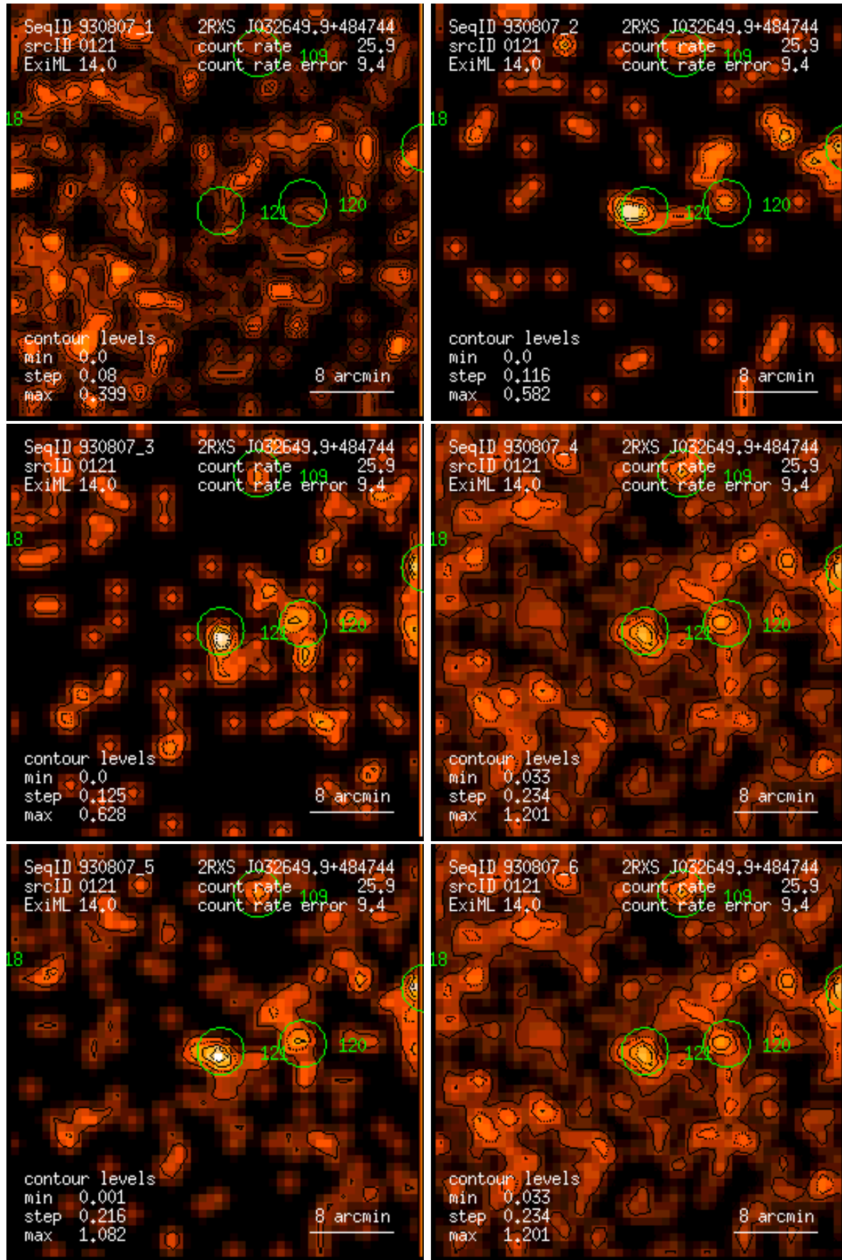
Figure 121: RASS 930807: detection 0121: band rate images, Gaussian filter: (1) PSPC channels 11 – 41, (2) 52 – 90, (3) 91 – 201, (4) 11 – 235, (5) 52 – 201, (6) 11 – 201. Broad band rates in counts/ks. Band rate contour levels in counts/ks/arcmin 2 .
