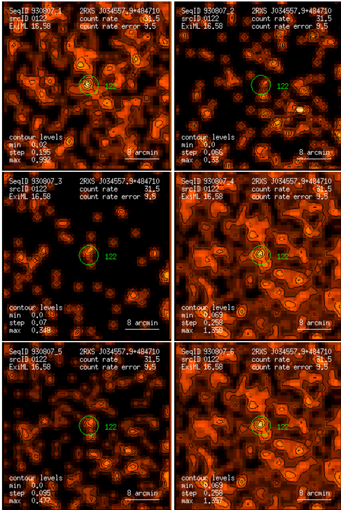
Figure 122: RASS 930807: detection 0122: band rate images, Gaussian filter: (1) PSPC channels 11 – 41, (2) 52 – 90, (3) 91 – 201, (4) 11 – 235, (5) 52 – 201, (6) 11 – 201. Broad band rates in counts/ks. Band rate contour levels in counts/ks/arcmin 2 .
