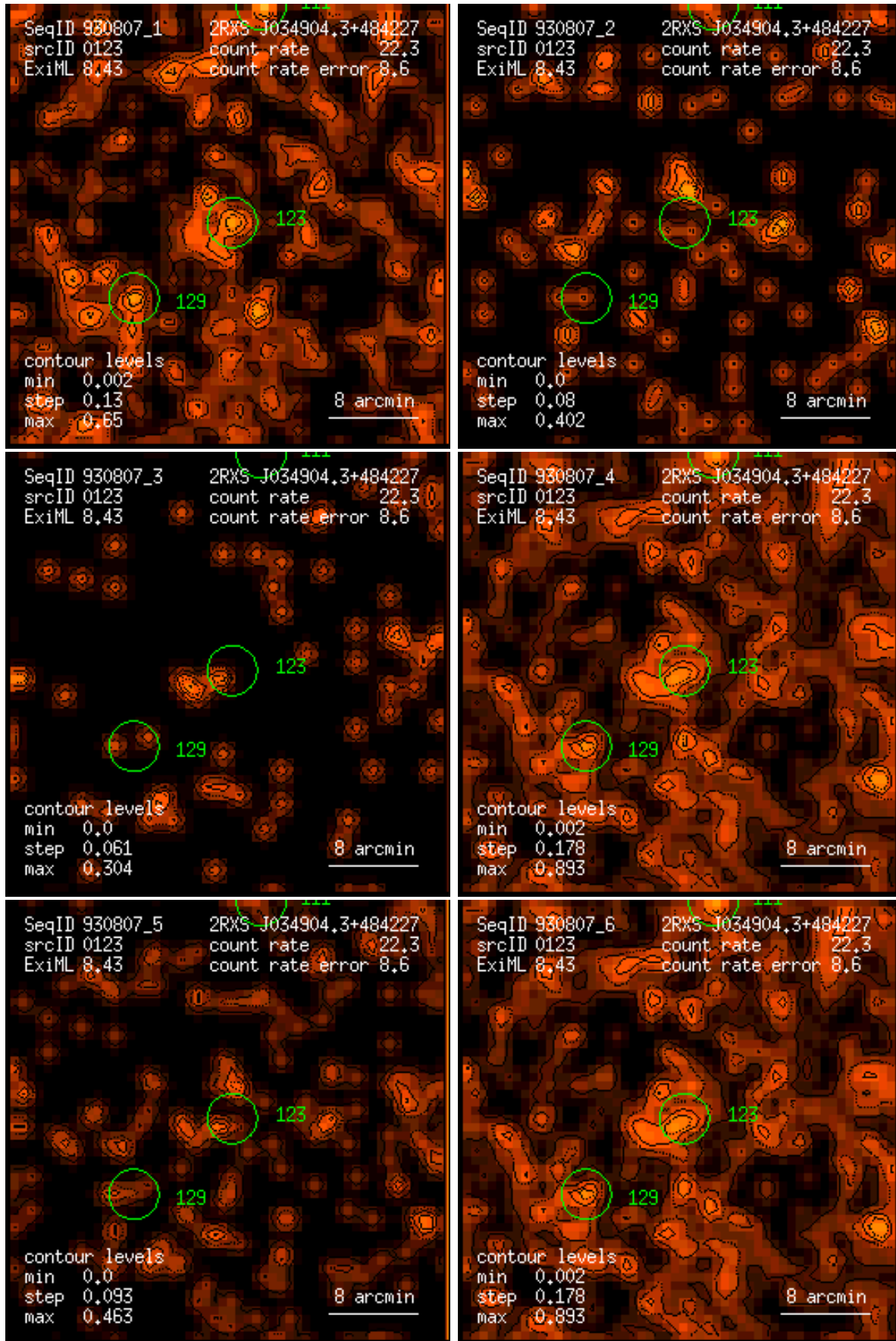
Figure 123: RASS 930807: detection 0123: band rate images, Gaussian filter: (1) PSPC channels 11 – 41, (2) 52 – 90, (3) 91 – 201, (4) 11 – 235, (5) 52 – 201, (6) 11 – 201. Broad band rates in counts/ks. Band rate contour levels in counts/ks/arcmin 2 .
