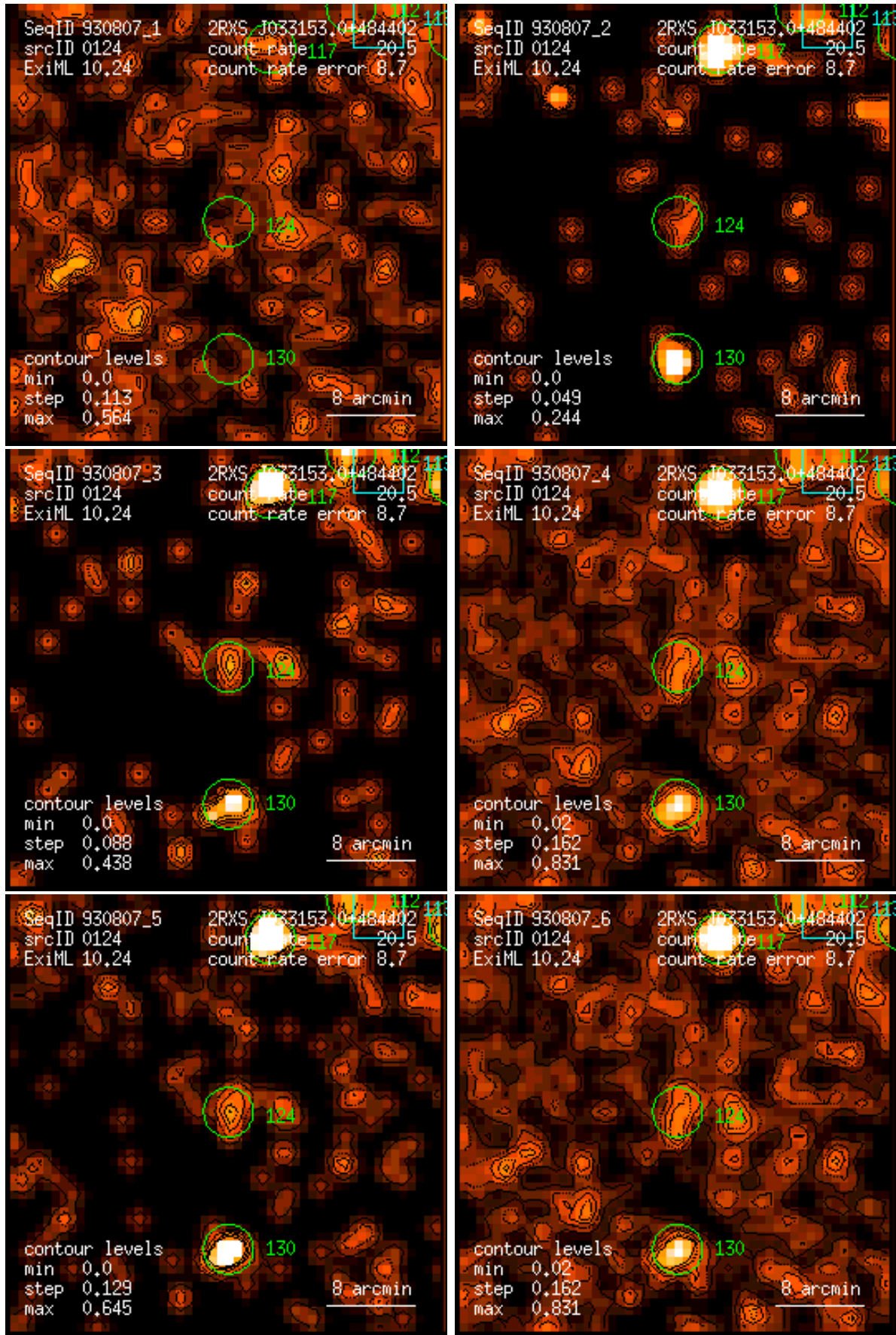
Figure 124: RASS 930807: detection 0124: band rate images, Gaussian filter: (1) PSPC channels 11 – 41, (2) 52 – 90, (3) 91 – 201, (4) 11 – 235, (5) 52 – 201, (6) 11 – 201. Broad band rates in counts/ks. Band rate contour levels in counts/ks/arcmin 2 .
