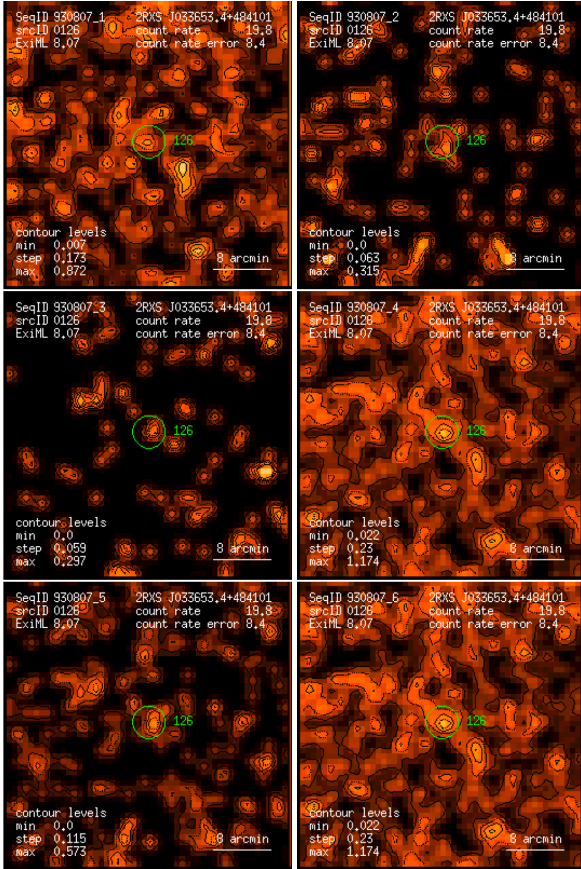
Figure 126: RASS 930807: detection 0126: band rate images, Gaussian filter: (1) PSPC channels 11 – 41, (2) 52 – 90, (3) 91 – 201, (4) 11 – 235, (5) 52 – 201, (6) 11 – 201. Broad band rates in counts/ks. Band rate contour levels in counts/ks/arcmin 2 .
