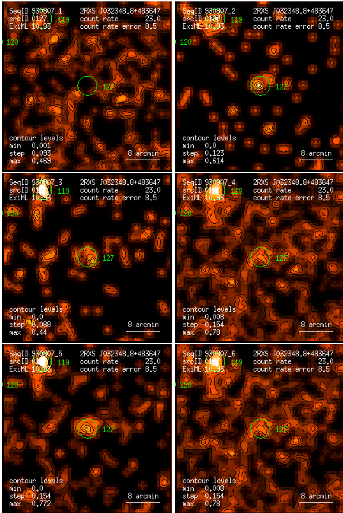
Figure 127: RASS 930807: detection 0127: band rate images, Gaussian filter: (1) PSPC channels 11 – 41, (2) 52 – 90, (3) 91 – 201, (4) 11 – 235, (5) 52 – 201, (6) 11 – 201. Broad band rates in counts/ks. Band rate contour levels in counts/ks/arcmin 2 .
